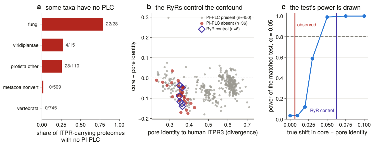
Extended Data Fig. 13 | The ligand core against the pore, and the lineages that lost the enzyme upstream.
