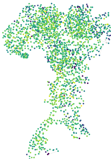
c ITPR3 (8TKG) resolves 2,210 residues
