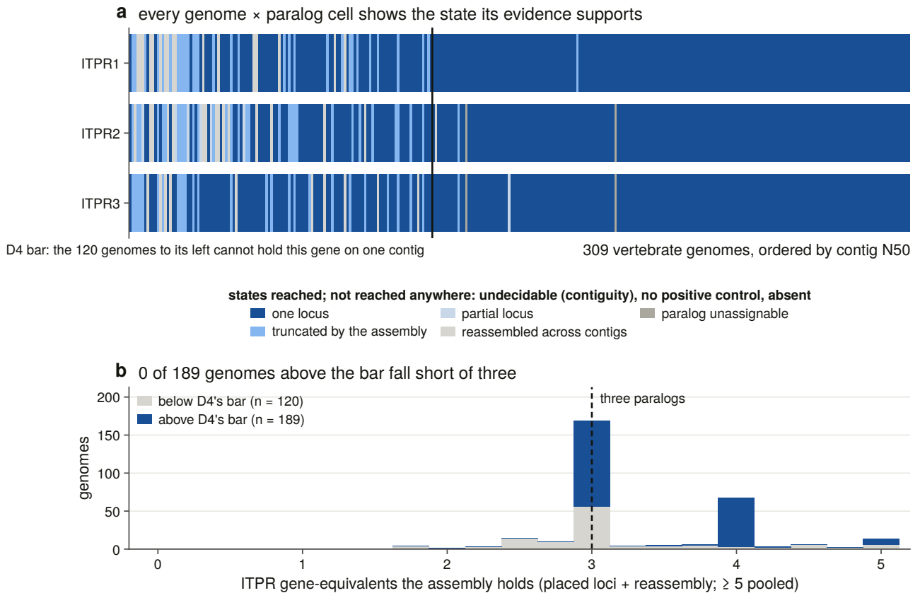
Fig. 5 | Three paralogues, retained in every vertebrate genome searched. (a) Every genome × paralogue cell, 309 genomes ordered left to right by contig N50, coloured by the state its evidence supports. The vertical line is the contiguity bar: the 120 genomes to its left cannot carry the gene on one contig. Three states are reached nowhere in the matrix and are named in the legend rather than drawn — undecidable for contiguity, no positive control, and absent. (b) The number of gene-equivalents each assembly holds, counting placed loci plus references reassembled across contigs, split by side of the bar. No genome above the bar falls short of three.
