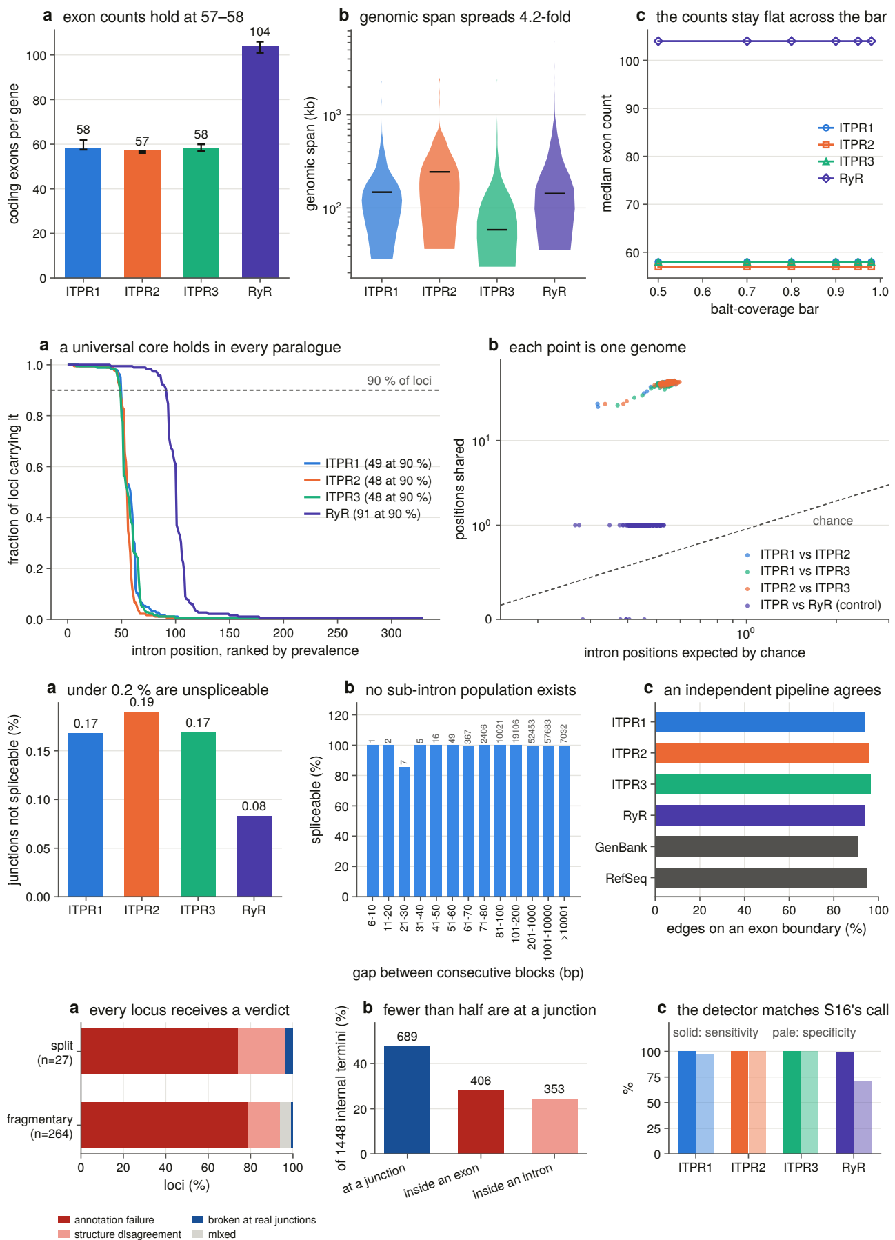
Extended Data Fig. 9 | The gene: exon structure, shared introns, and where a fragmentary annotation stops. (a) Coding exons per gene (median with 10th–90th percentiles), genomic span per locus on a logarithmic axis, and the median exon count recomputed at six coverage bars, for the three paralogues and the ryanodine
