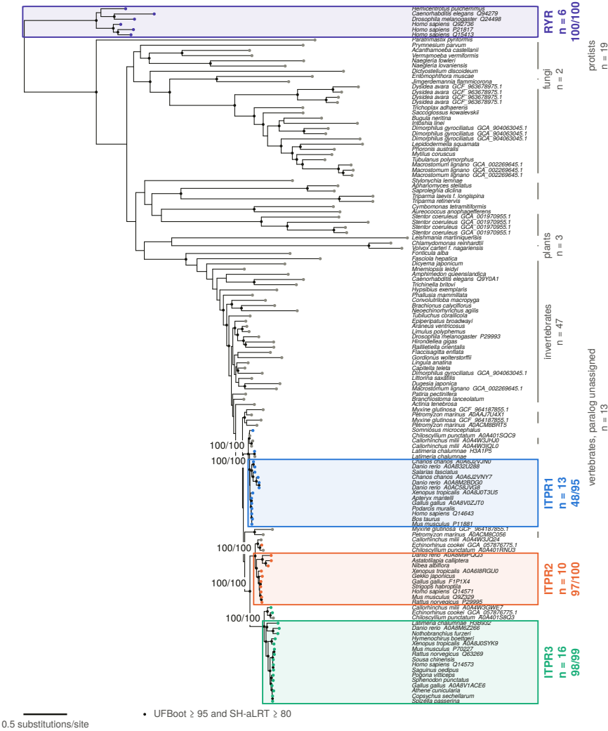
The maximum-likelihood tree of 134 family proteins recovers ITPR1, ITPR2 and ITPR3 as clades, rooted on the ryanodine receptors
