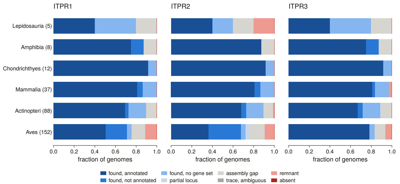
Fig. 2 | The three-paralogue census across 309 vertebrate genomes. Evidence class for each of ITPR1 , ITPR2 and ITPR3 in every genome, stacked as a fraction of the genomes of each vertebrate class that the scope samples more than once — six classes and 302 of the 309 genomes (class sizes in brackets). Darkest blue is a locus found and correctly annotated; the next two blues are a locus found in an assembly whose annotation misses it or that has no gene set at all; the palest blue is a locus recovered only in part; grey is an assembly gap and the darker grey an ambiguous translated trace; salmon is a remnant recovered only by translated search. The absent colour appears nowhere because the four cells that carry it — both cyclostomes’ ITPR2 and ITPR3 — are the only two genomes of their classes and those classes are not drawn; S15 re-states those four cells as paralogue-unassignable, for the reason given in the text. Aves carry the most non-blue cells of any class and are the least contiguous class in the scope; the largest non-blue fraction is Lepidosauria’s, on five genomes.
