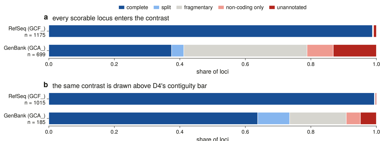
Fig. 7 | How the family is recorded, and by whom. Annotation state of every scorable IP 3 receptor locus, split by whether the assembly's annotation came from RefSeq or from the submitter through GenBank. (a) All 1,874 scorable loci: RefSeq is 98.8 % complete and GenBank 37.5 %. (b) The same contrast restricted to loci on a contig long enough to hold the gene, which removes assembly quality as an explanation and leaves 99.4 % against 63.8 %. The archive an assembly is deposited in predicts whether its IP 3 receptor is recorded far better
