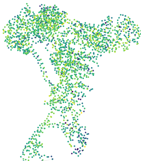
a ITPR1 (7LHF) resolves 2,300 residues
