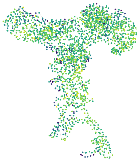
b ITPR2 (9YKK) resolves 2,168 residues
