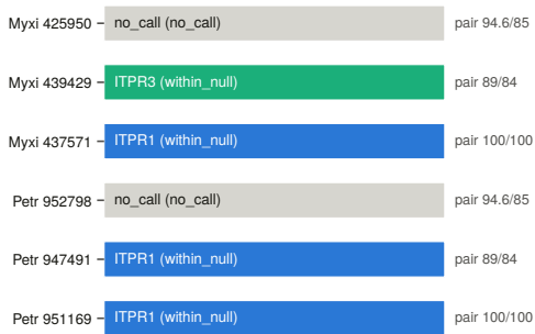
b S8's flanks call 4 of 6 loci; 2 get no call
