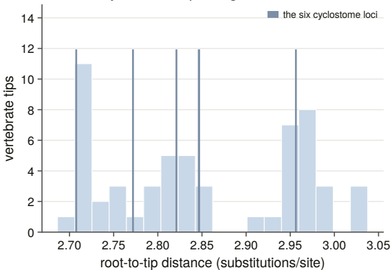
a Are the cyclostome tips long branches?
