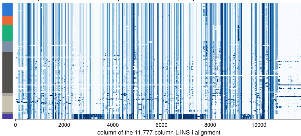
a 134 representatives are drawn as per-cell residue occupancy
