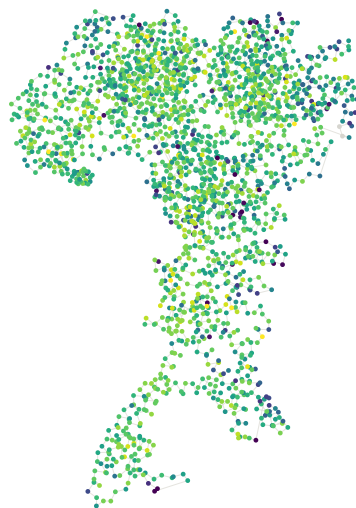
c ITPR3 (8TKG, 2,210 resolved residues)
