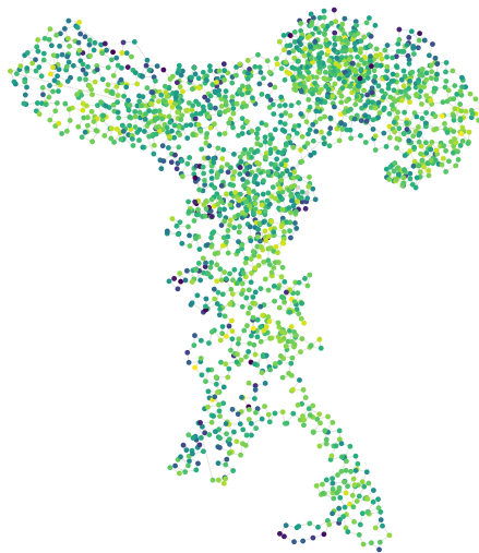
b ITPR2 (9YKK, 2,168 resolved residues)
