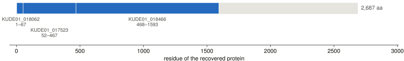
Figure 13.7. The annotated proteins tiled back onto the genome’s own recovered loci. The proteins are translated from the assembly’s own annotation and genome rather than downloaded, because a locus filed as a pseudogene emits no protein record and the only way to ask what its model encodes is to translate it. The guard that matters is that the subject set is the genome’s own loci: a query whose own locus is missing from the subject set lands on its nearest paralogue instead, and the row then reads as a confident naming disagreement, which is exactly what happened before the check existed.
