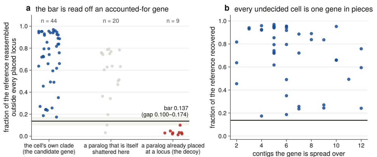
Figure 9.2. The three populations the bar is read off, with the gap shaded and the operating point drawn, and every undecided cell against the number of contigs its gene is spread over. A calibration figure that asked to be believed would not be one, so both edges of the gap are marks rather than a caption.
