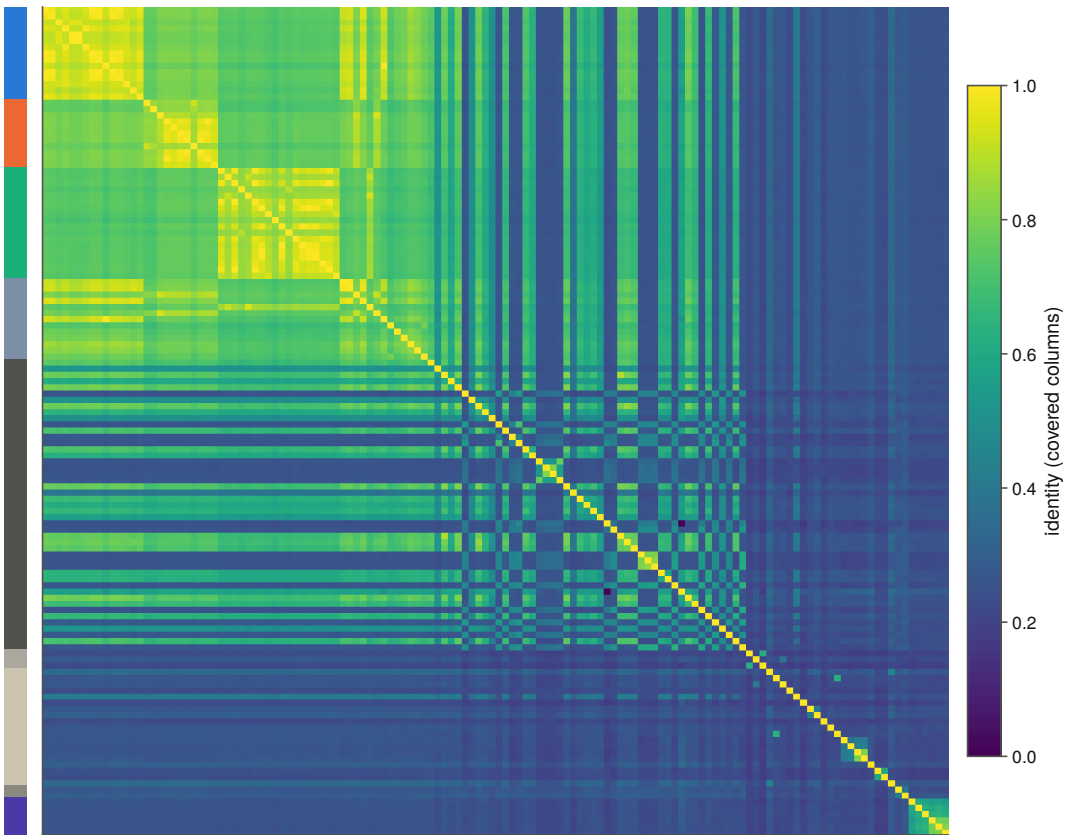
Pairwise identity over mutually covered columns, 134 representatives
