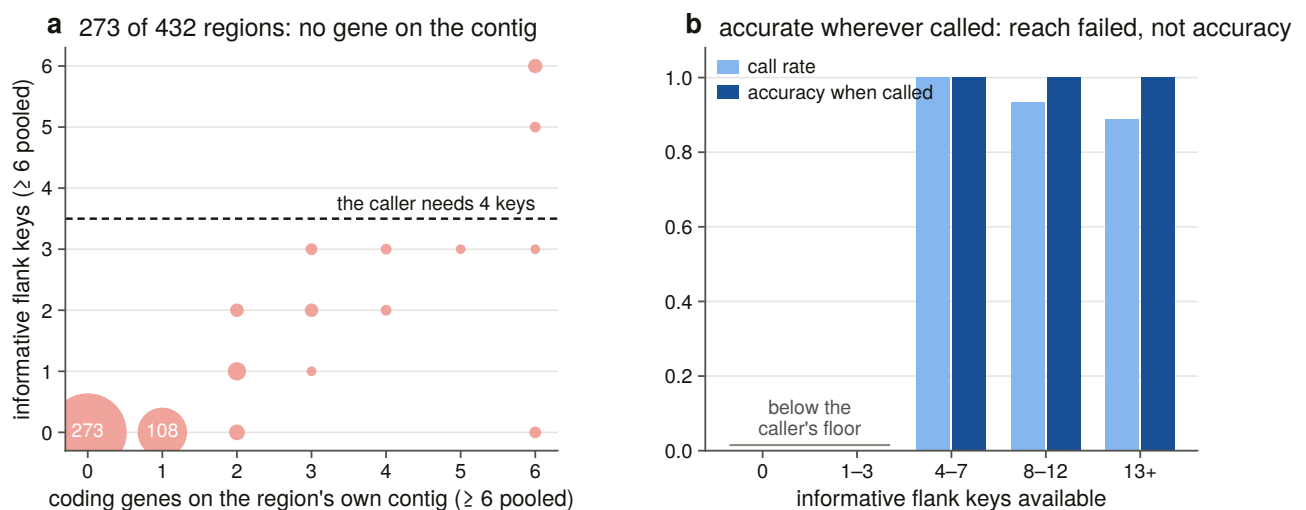
Figure 9.4. Why synteny could not answer, showing the joint distribution of what a trace region has to work with, with the caller's floor drawn, beside the caller's own accuracy on the same axis. Putting reach and accuracy on one axis is what makes "accurate and unavailable" a readable sentence rather than an excuse.
