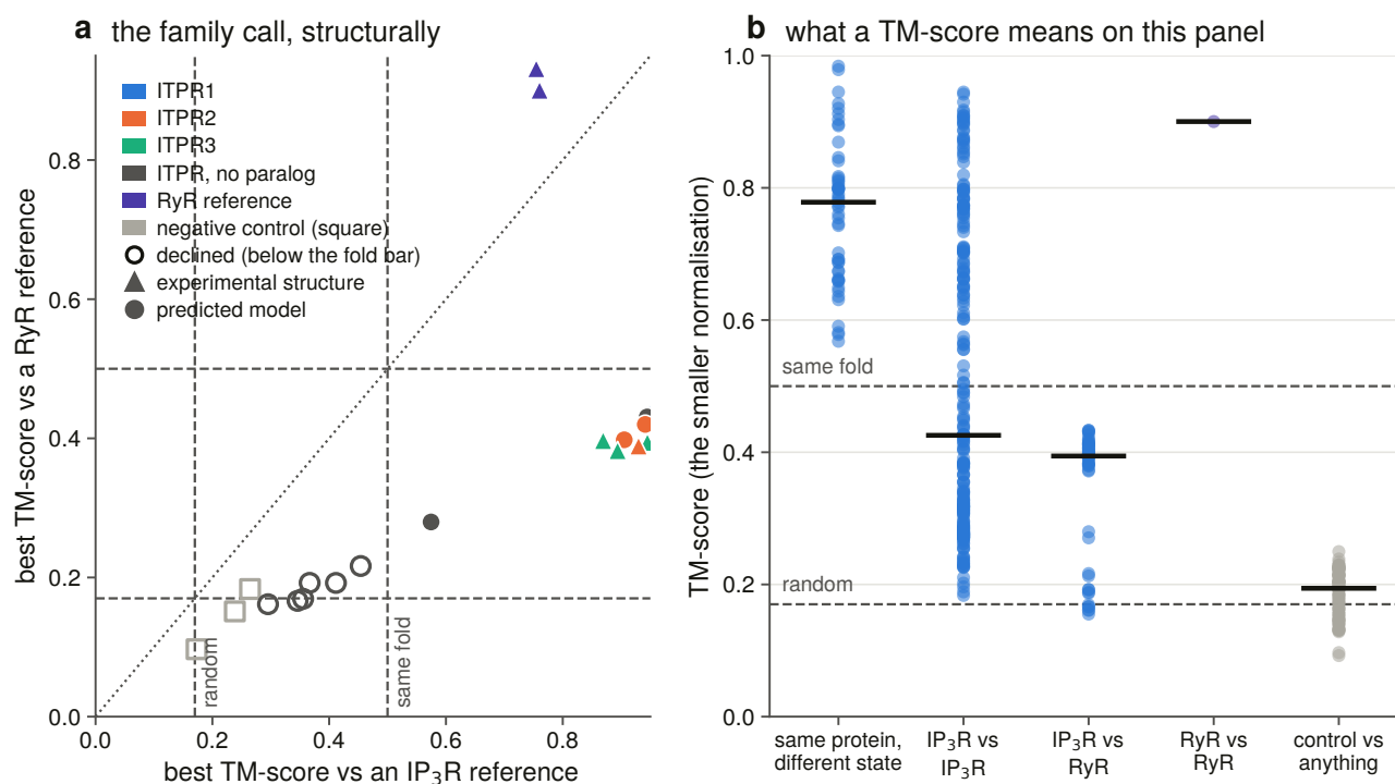
Figure 11.2. The family call made structurally, and the calibration behind it. Both of the alignment method’s published bars are drawn, meaning the random-similarity floor and the same-fold bar [74], rather than described. A calibration figure that asked to be believed would not be one.
