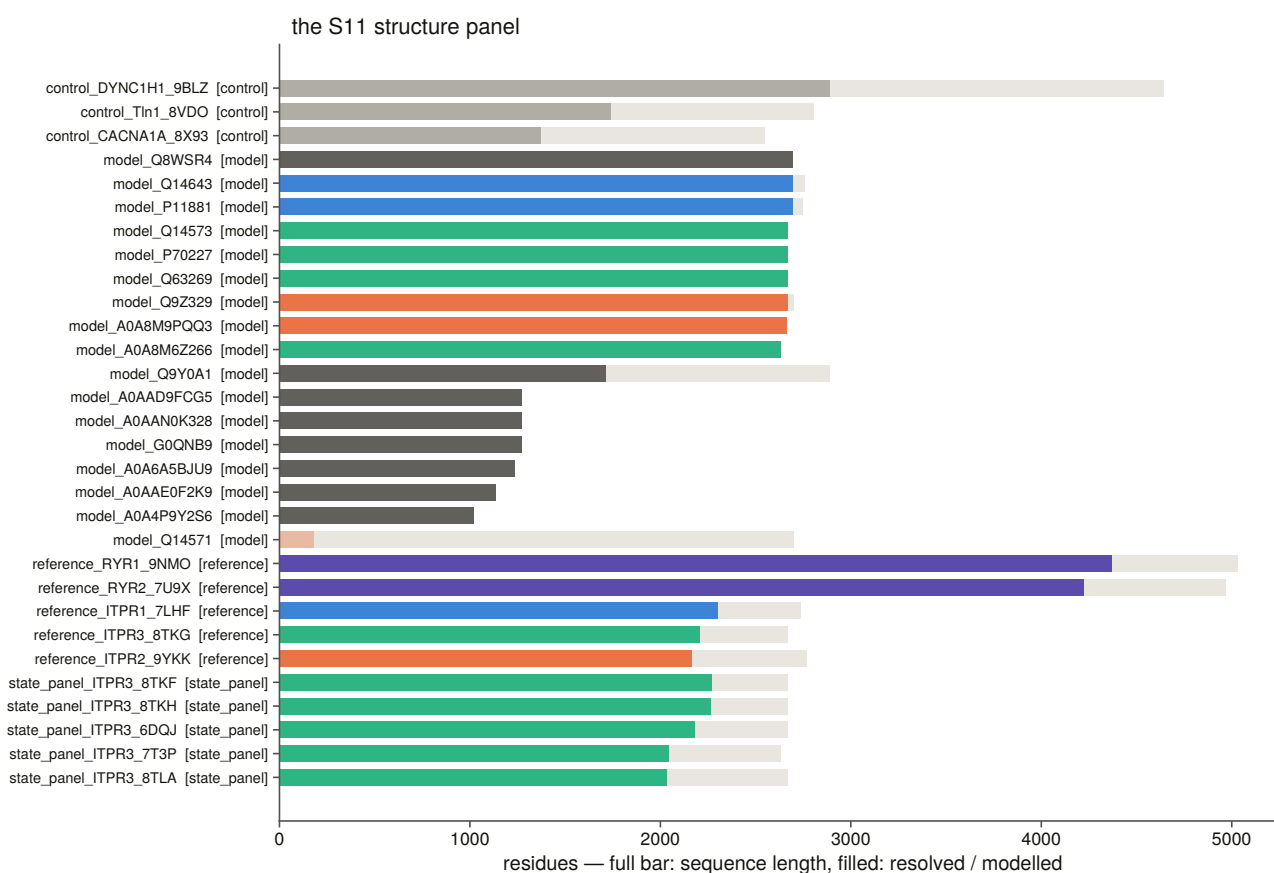
Figure 11.1. Every structure in the panel, where the pale bar is the length the record claims and the filled bar what the structure delivers.
