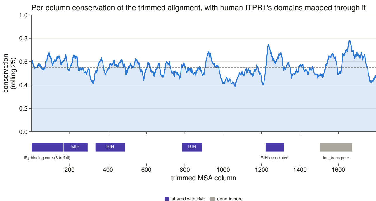
Figure 6.1. Per-column conservation with human ITPR1’s domain architecture mapped onto it through the alignment, by walking the human row and counting ungapped positions, rather than by scaling residue coordinates onto column coordinates. The latter is the mistake that puts a domain boundary in the wrong place by exactly the gap content of the sequence.
