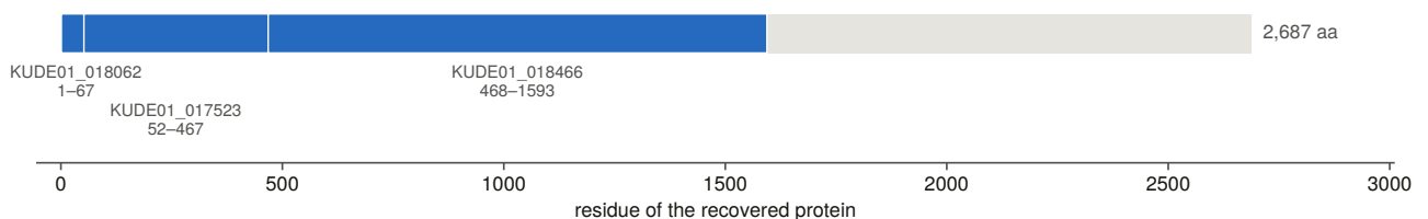
Figure 13.7. The annotated proteins tiled back onto the genome's own recovered loci. The proteins are translated from the assembly's own annotation and genome rather than downloaded, because a locus filed as a pseudogene emits no protein record and the only way to ask what its model encodes is to translate it. The guard that matters is that the subject set is the genome's own loci: a query whose own locus is missing from the subject set lands on its nearest paralogue instead, and the row then reads as a confident naming disagreement, which is exactly what happened before the check existed.
