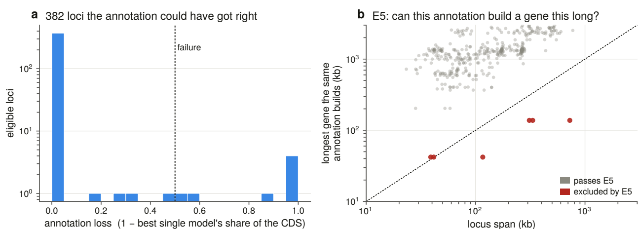
Figure 13.6. Annotation loss across every recovered locus, which is the denominator the two cases are chosen from: 880 loci, 382 eligible, and 360 of them at zero loss.
