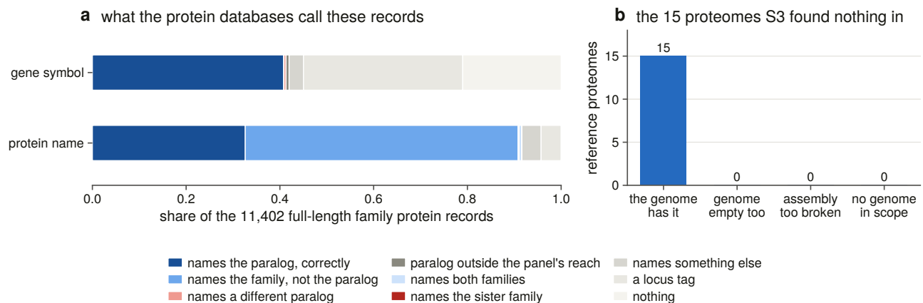
Figure 13.4. The protein records, showing what the name claims against what the sequence is.
