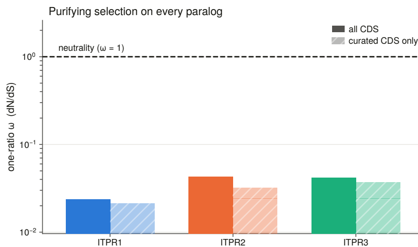
Figure 10.1. Per-paralogue rate with the curated-sequence sensitivity estimate beside it, and neutrality drawn rather than described. The axis is logarithmic, because at a rate of 0.03 a linear axis puts every bar on the floor and hides the one thing a reader wants, which is how far below one it sits.
