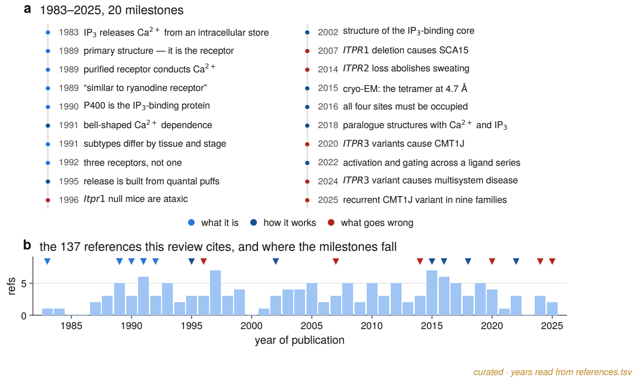
Figure 1.5. Four decades of work on the receptor as the literature records it, with each milestone drawn at the year of its published source. The figure is generated from a curated table in which no year is typed: each is read from the reference row it cites, so a milestone cannot be dated differently from the paper it rests on. The density on the right is the cryo-electron microscopy era, which is what made the structural half of this project possible.
