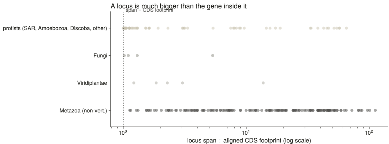
Figure 5.8. Locus span against coding footprint, by group. A locus is much larger than the gene inside it, and by a factor that varies by group, which is the reason the intron parameter is set per group and the reason a locus is not a copy.
