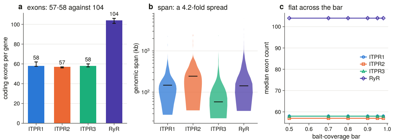
Figure 8.1. Exon count and genomic span on separate axes, with span logarithmic and count not. The result is that one is conserved and the other is not, and a shared scale would hide it.
