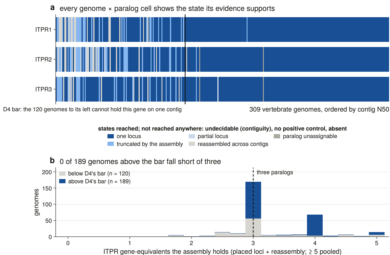
Fig. 5 | Three paralogues, retained in every vertebrate genome searched. (a) Every genome × paralogue cell, 309 genomes ordered left to right by contig N50, coloured by the state its evidence supports. The vertical line is the contiguity bar: the 120 genomes to its left cannot carry the gene on one contig. Three states are reached nowhere in the matrix and are named in the legend rather than drawn — undecidable for contiguity, no positive control, and absent. (b) The number of gene-equivalents each assembly holds, counting placed loci plus
