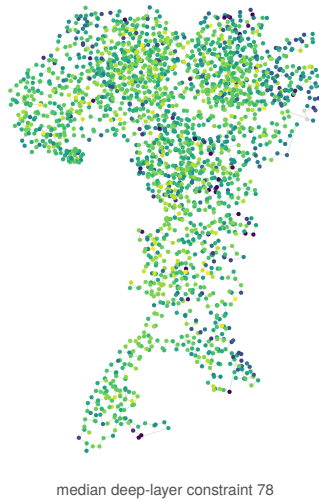
c ITPR3 (8TKG) resolves 2,210 residues
