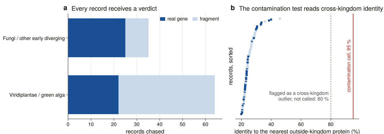
Figure 5.3. The chase of every plant and fungal record ends in a verdict, and the cross-kingdom identity that the contamination test rests on is plotted for each record. That axis decides whether these records are biology or contamination, which is the question the whole range claim turns on: a genuine deep homologue is 20 to 40 % identical to its metazoan relatives, while an assembly contaminant is 95 to 100 % identical to one particular animal. Nothing here is above 40 %, so the surviving records are real green-algal and early-diverging fungal genes, which is what makes the land-plant and Dikarya absences losses rather than the family's boundary.
