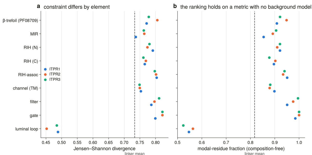
Figure 11.6. Constraint is ranked by element on the divergence metric in panel a and on the composition-free metric in panel b, beside it rather than instead of it. The headline result and its most obvious artefact are therefore on the same axis: the gate comes first or second on both metrics and the filter stays in the top four, so the ranking is not a property of one scoring choice, and a reader can check that agreement rather than take it on assurance. The second metric is there because a divergence from a background frequency table [93] scores a transmembrane element lower at equal conservation, which would have manufactured the very result the chapter reports.
