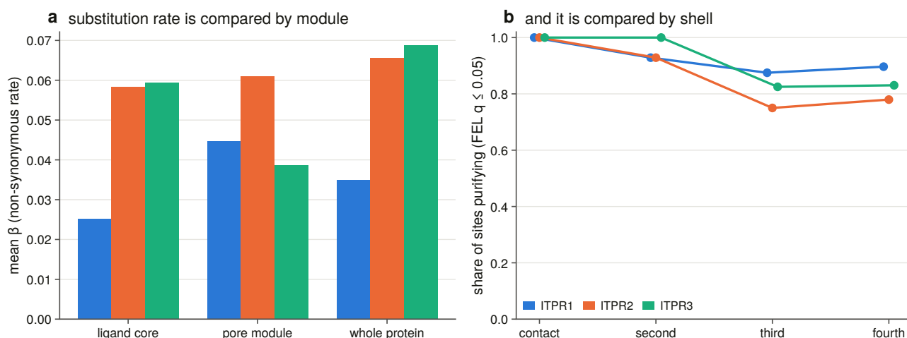
Figure 12.4. Per-site substitution rates are compared by module in panel a and by shell in panel b. The importance of this figure is that it asks the same question with a different quantity. A column's dispersion across orthologues and a site's substitution rate on a tree are both called constraint and are not the same measurement, so a result that appears on one axis and not the other is bounded rather than confirmed. The contact result replicates here and the module comparison does not, and the figure is where that distinction is visible.
