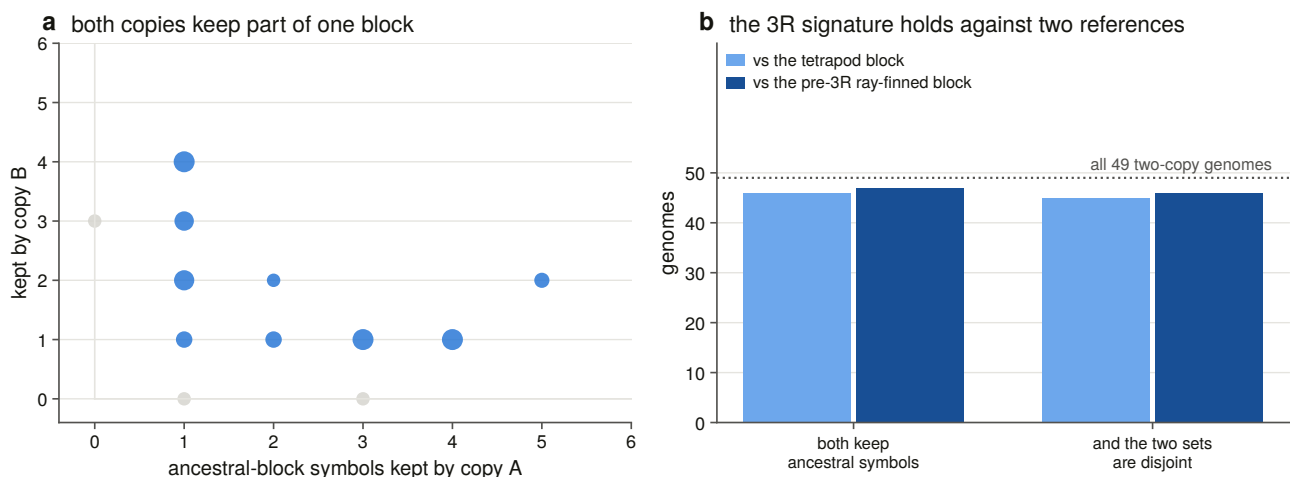
Figure 7.11. Double-conserved synteny is shown by plotting the two copies against each other, so that disjointness is a geometric fact on the figure rather than a number in a table. The load-bearing word in this figure is disjoint. Two copies that each resemble the ancestral neighbourhood could be two independent later duplications, but two copies that partition it between them are what reciprocal gene loss after a single duplication produces. That distinction is what turns a copy count into a claim about one shared event.
