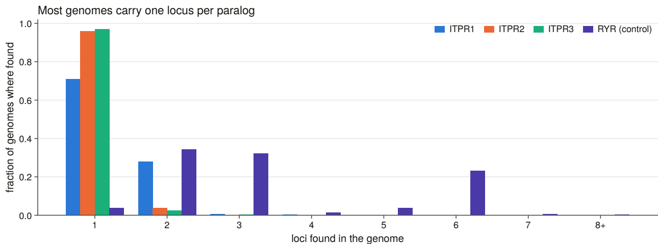
Figure 4.4. The figure counts the family's loci per genome across the sweep. The excess above three copies is not spread across the vertebrates but sits almost entirely in the ray-finned fish, which is what a whole-genome duplication confined to one lineage looks like from a copy count. Chapter 7 turns that observation into a tested claim about which paralogue was doubled and retained.
