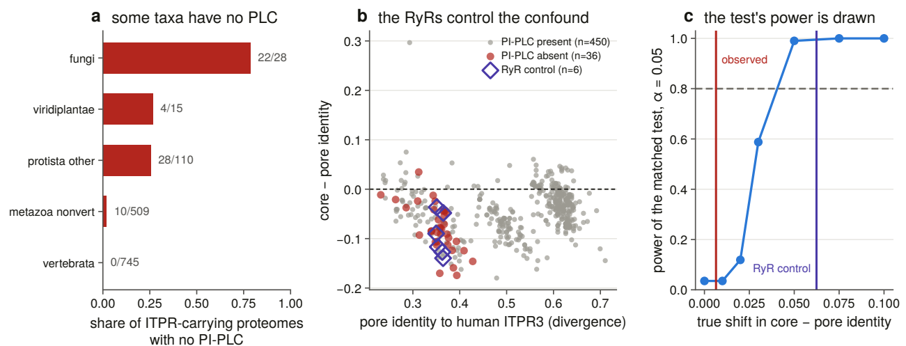
Figure 12.5. The lineage strata are drawn with the power curve beside them, which is what makes a negative result readable: panel a compares receptors with and without the enzyme, panel b shows the divergence confound and the ryanodine control, and panel c shows what the test could have seen. Lineages that lost the enzyme making the ligand show no relaxation at the binding site, and without a bound on what the comparison could have detected that would be an untestable statement. The ryanodine receptors are the positive control, because they carry the same pore and no ligand site, so the shift the design can see is measured rather than assumed. The ligand core is drawn in a neutral dark rather than a hue, because the palette reserves its accent colour for that control.
