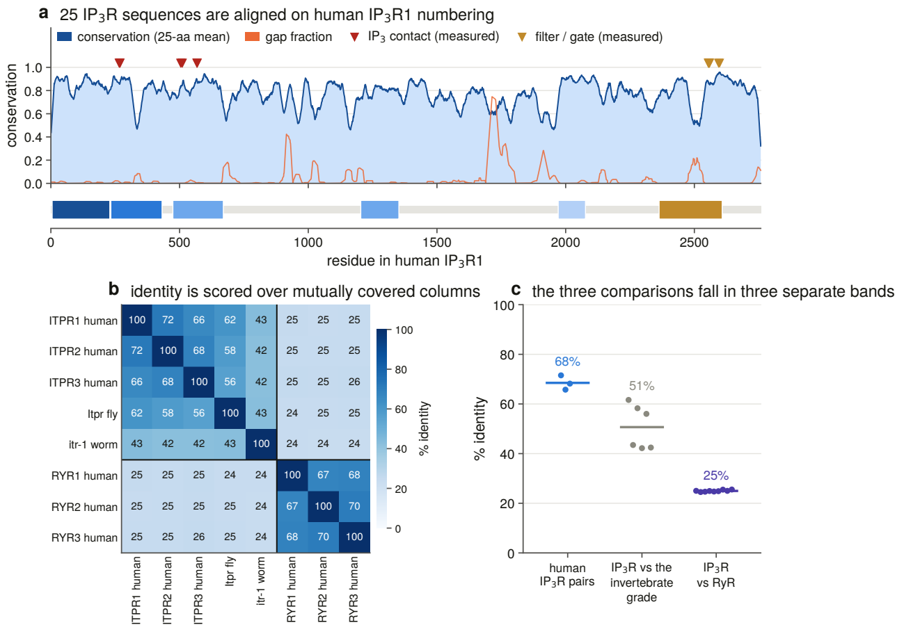
Figure 2.5. Conservation is plotted per column across a 25-sequence family alignment, mapped onto human ITPR1 numbering, with the domain architecture beneath it. (a) The smoothed profile runs along the human sequence. (b) The matrix gives identity over mutually covered columns for every pair. (c) The three comparisons that matter are drawn as distributions. Chapter 11 rebuilds this at a very different depth, using 249 to 265 orthologues of each individual paralogue rather than 25 sequences of the whole family, and the two agree about where the peaks are. That agreement matters for a practical reason: if a shallow family alignment and a deep within-paralogue alignment disagreed about where the receptor is conserved, neither could be used to interpret a clinical variant. It is what licenses Chapter 11 to compare four conservation layers as classifiers rather than to pick one on faith.
