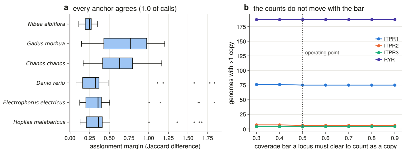
Figure 7.12. Cross-anchor block identity is shown beside the sensitivity of every copy count to the coverage bar. Seven bars are scanned, because a duplication claim that survives only one bar is a claim about the bar. The anchor panel is what separates one ancestral duplication from a series of lineage-specific ones, which the copy counts alone cannot do, because anchors from six different orders assign every genome independently and would carry no shared information if each lineage had duplicated on its own.
