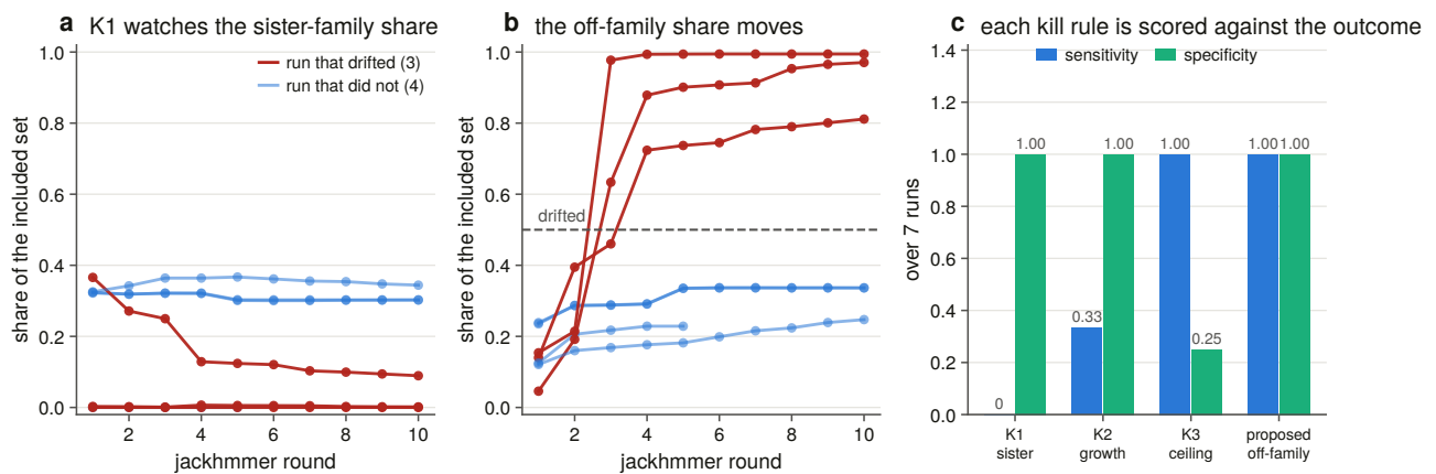
Figure 4.8. Each kill rule is scored as a classifier of a drift outcome that was measured on the finished model. The figure records an instrument failing at the one job it was built for: the rule written to catch sister-family drift has a sensitivity of zero across seven runs, including all three that drifted, because the drift dilutes the very quantity the rule measures. The correction is a one-line change to a different axis, and it is reported rather than applied, because it was validated after the fact on the runs it would reclassify.
