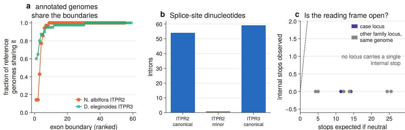
Figure 13.8. Three of the five checks on each case are drawn together, and none of them fails. In panel a, every internal exon boundary of each case is ranked by the fraction of independently annotated reference genomes that share it. Panel b counts the introns of each locus by their splice-site dinucleotides. Panel c plots the internal stops observed in each case locus, and in every other family locus of the same genome, against the stops expected if the sequence were drifting neutrally. Showing the checks together matters because no single one of them is decisive: splice dinucleotides, an intact reading frame and exon-boundary concordance each fail in different circumstances, and they do not fail together, so a reader asking whether a recovered gene is an alignment artefact is asking whether every one of these could be wrong at once.
