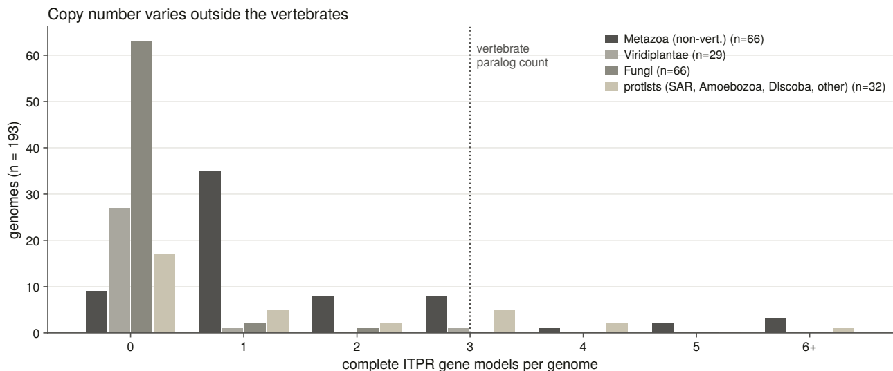
Figure 5.6. Copy number outside the vertebrates runs from zero to eighteen, and the vertebrate paralogue count is drawn as a reference line rather than as a category. Drawing it that way shows the vertebrate three to be unremarkable: a flatworm carries eighteen receptors and a ciliate thirteen, so copy-number expansion in this family is not a vertebrate story and three is not the family's high-water mark. What is specific to the vertebrates is that their three copies are ancient, distinct and universally retained.
