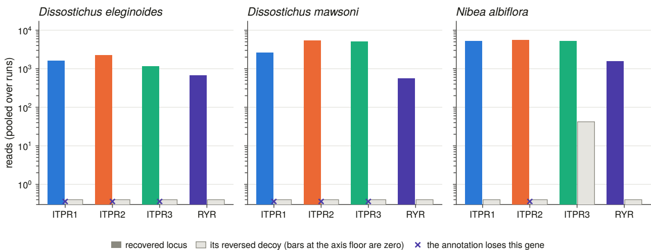
Figure 13.9. Every recovered locus collects reads far above its own reversed decoy. Each panel is one species, with the pooled read count on each of its four family loci drawn beside the count on a decoy of identical length and composition, and a cross marks each locus the annotation loses. The decoy replaces a chosen cut with a measured one: a sequence with no homology collects whatever this reference collects by accident, so a locus above its own decoy is detected on evidence. Counts are on logarithmic axes because these libraries differ roughly forty-fold in depth, and the comparison that means anything is between a locus and its decoy in the same run.
