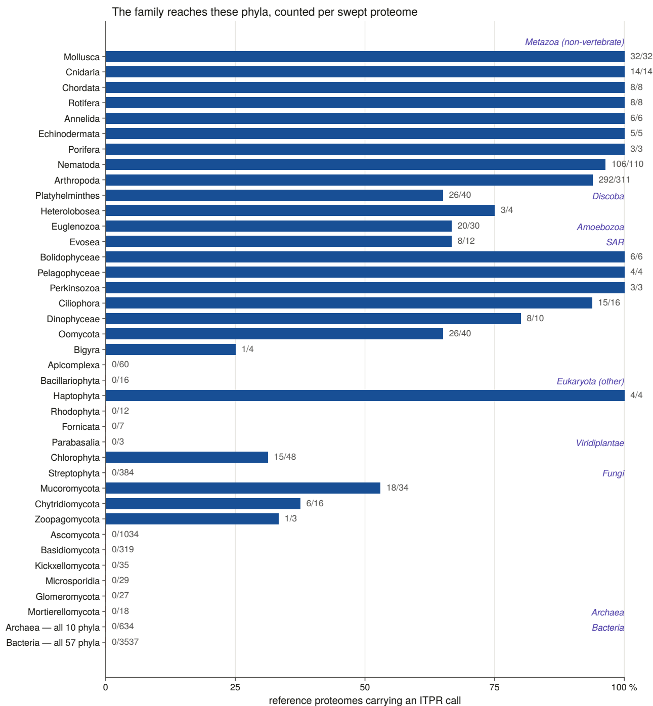
Figure 5.1. The family's presence across the eukaryotes is drawn as a fraction of swept proteomes rather than of records. That denominator is the whole point: counted by records, a single well-sequenced alga outvotes a sparsely sampled phylum, and the figure would report sequencing effort. The importance of this figure is the shape rather than any single bar. A family present across the metazoa, in several protist lineages, in the green algae and in the early-diverging fungi, and absent from land plants and from the yeasts and moulds, is a family that was present in the eukaryotic ancestor and has been lost repeatedly since. That is a different claim from an animal innovation, and it is what the figure supports.
