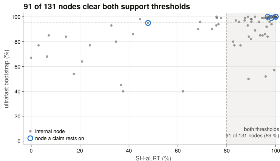
Figure 6.9. Node support is drawn as a scatter of the two branch tests rather than as two histograms, because the claim is about the joint condition and a pair of marginals cannot show it. A node is trustworthy here only when both branch tests agree. The bootstrap alone is known to be optimistic under model violation, which a 134-tip alignment spanning four kingdoms guarantees, so every well-supported claim in this thesis requires both.
