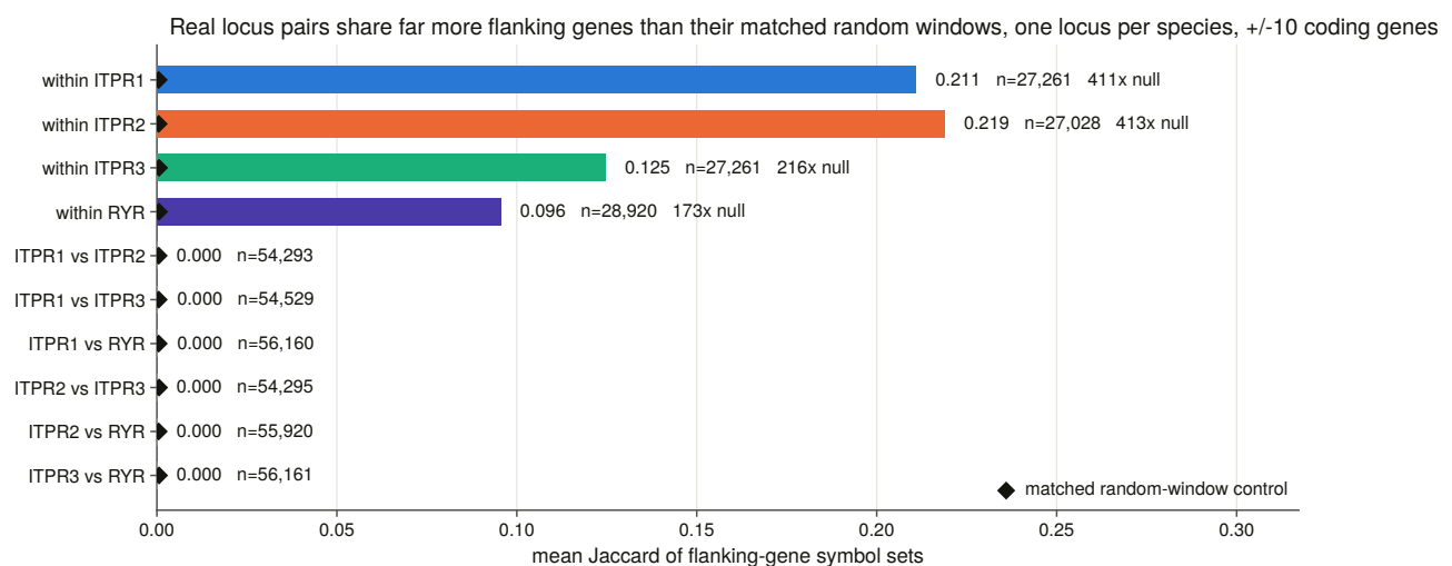
Figure 7.1. Each pair class stands beside its matched random-window control, and the three within-paralogue classes clear theirs by two orders of magnitude while every class that crosses a paralogue or the family boundary sits at or below its own. The paralogue cells were assigned from sequence, and no earlier chapter had checked them against evidence outside the gene itself, so this is the first test of an assumption every chapter since Chapter 3 has made. Its bearing for a reader is that the cells can be read as orthology groups rather than as bins of similar sequence.
