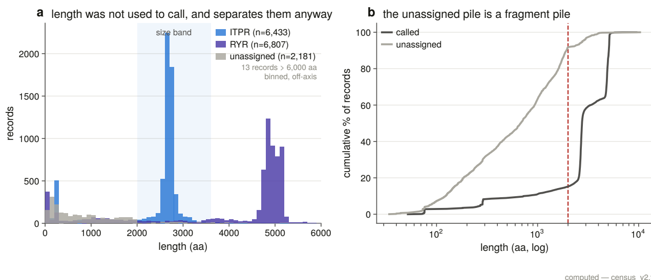
Figure 3.4. The two families separate cleanly by length as called. (a) The medians are 2,671 and 4,856 residues and the distributions barely touch. (b) The records neither test could call sit far below both families in length, which is what a pile of fragments looks like. The figure shows why a filter that works is still not evidence: length separates the two families almost perfectly here, and it does so on a population whose annotations are already good, which is precisely where no separation is needed. In the fragmentary and unannotated records where the call actually matters, this separation is unavailable, and a project that had trusted it would have inherited annotation quality as a definition of the gene family.
