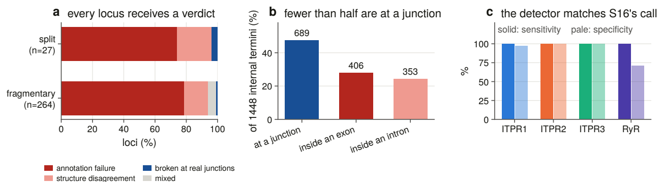
Figure 8.4. Most fragmentary annotations have at least one end inside an exon, and the duplication detector agrees with an independent copy call. Panel a gives the verdict for every split and fragmentary locus, panel b places the annotation's internal termini relative to the gene model, and panel c scores the detector against the copy call. The first two panels convert a database label into a testable claim: a locus called fragmentary might have been annotated as a plausible short gene, or the annotation might have stopped where no splicing machinery could stop, and only the second is an error. 228 of 291 such loci carry at least one terminus in the middle of an exon, which falsifies the innocent reading. The third panel makes the same point about an instrument, since scoring the detector against a copy call it never sees moves its specificity from 0.16 to 0.977 once the family assignment is applied first.
