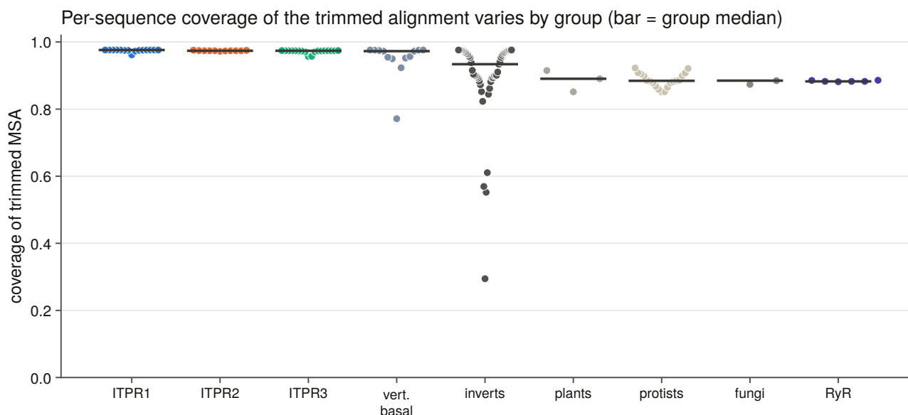
Figure 6.2. Each representative's coverage of the trimmed alignment is plotted by group, with a bar at each group's median. The median is 0.96 and one tip of 134 covers less than half. Coverage matters because a tip that covers half the alignment contributes gaps to every column the tree is inferred from, and gaps are not neutral for a likelihood model. Naming that one tip, rather than reporting only the median, is what allows a reader to judge whether any deep node depends on it.
