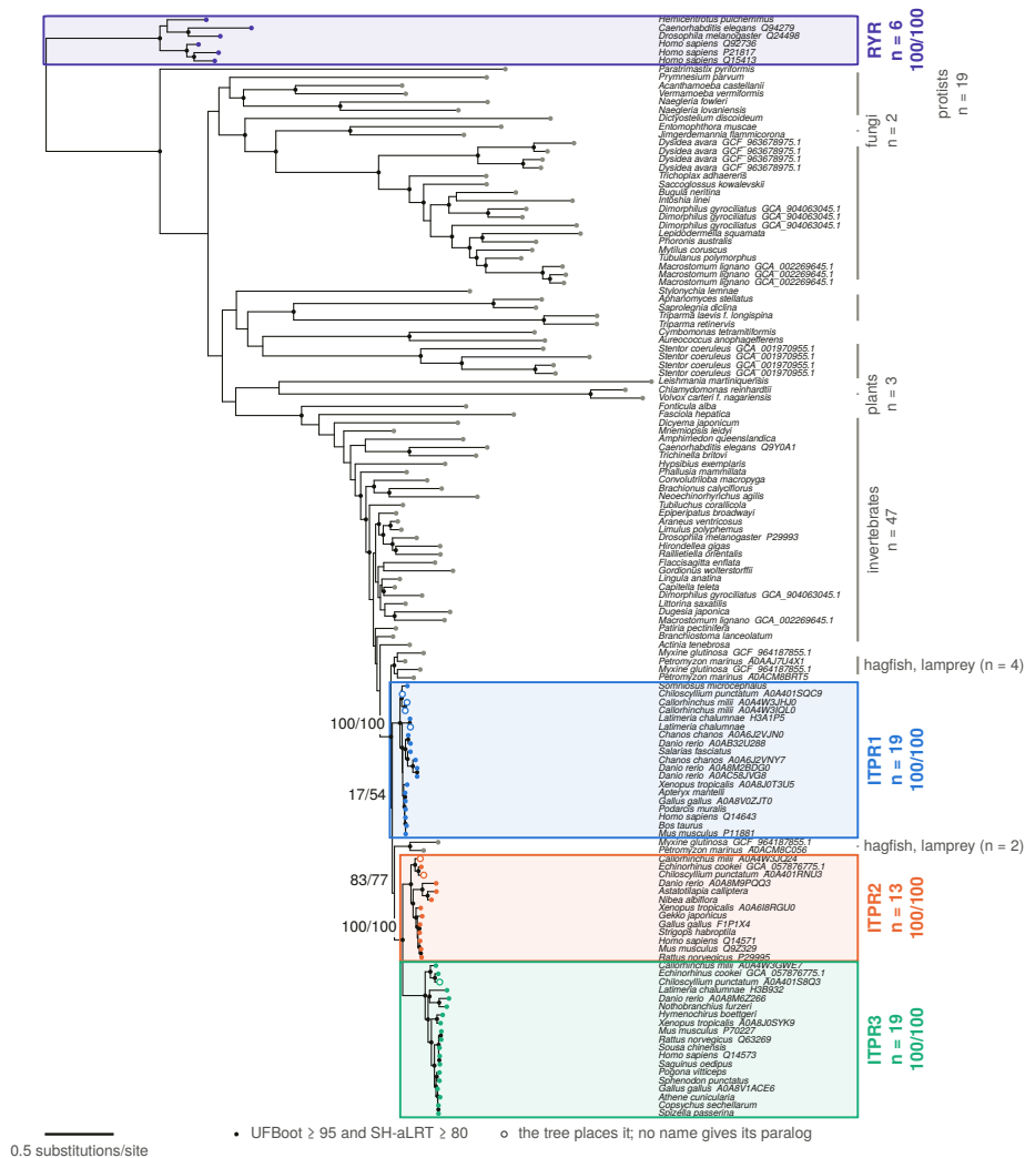
Figure 6.6. The rooted maximum-likelihood phylogram places all 134 representatives, and every protein outside the purple box at the top is an IP_3 receptor; the purple box holds the six ryanodine receptors that root the tree. Each coloured box is one paralogue's whole clade, which holds 19 proteins for ITPR1 , 13 for ITPR2 and 19 for ITPR3 , and each clade is supported at 100/100 (SH-aLRT/UFBoot), as printed beside its box. A filled coloured dot marks a protein whose database record names its paralogue. An open circle marks one of seven proteins from sharks, a chimaera and the coelacanth whose records do not say which paralogue they are; the tree places four of them in ITPR1 , two in ITPR2 and one in ITPR3 . Counted on names alone, the ITPR1 core is only 13 tips at 47.8/95, because the unnamed shark and coelacanth genes sit interleaved at its base, so the paralogue is well supported only once they are counted. The six grey vertebrate proteins outside the boxes are from hagfish and lamprey, and their paralogue cannot be assigned: four form their own clade (99.5/100) that branches first among the 57 vertebrate proteins, and two join the ITPR2 + ITPR3 clade at 83.1/77, below the joint bar. Both groups hold hagfish and lamprey genes together, which is why §6.9 reads them as two lineages older than the split between those two fish. The grey proteins above the vertebrates are invertebrate, protist, plant and fungal receptors, bracketed and counted on the right; they carry no paralogue because the three paralogues arose inside the vertebrates. Numbers on the backbone are the supports of the nodes that join the clades, and the two weak ones are the nodes where the jawless-fish proteins attach. A filled black dot marks every node clearing both SH-aLRT \geq 80 and UFBoot \geq 95 . No tip is ringed, because the relabelling rule described in §6.7 fires on none of them. The tree matters because it answers a question the literature had left open: the review's own audit found no published, support-annotated maximum-likelihood analysis with a ryanodine outgroup that fixes which two of the three paralogues are sisters.
