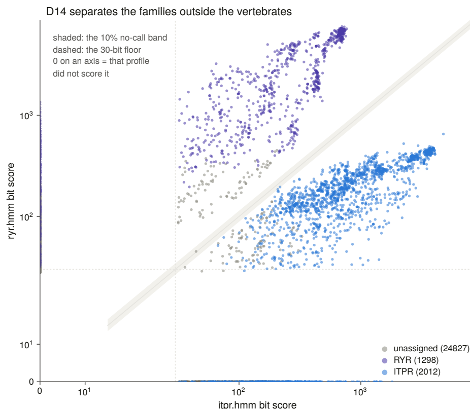
Figure 5.2. The same two-profile separation holds outside the vertebrates, and the no-call band is drawn on the figure. 28,137 targets were scored by at least one profile and 2,769 by both above the floor, which are the only ones where the two families can be said to compete at all, and exactly one of those falls inside the band where the instrument declines to choose. The family separation therefore transfers intact to organisms a billion years of divergence away from where it was calibrated. Without that, every non-vertebrate count in Chapter 5 would be a mixture of two families rather than a measurement of one.
