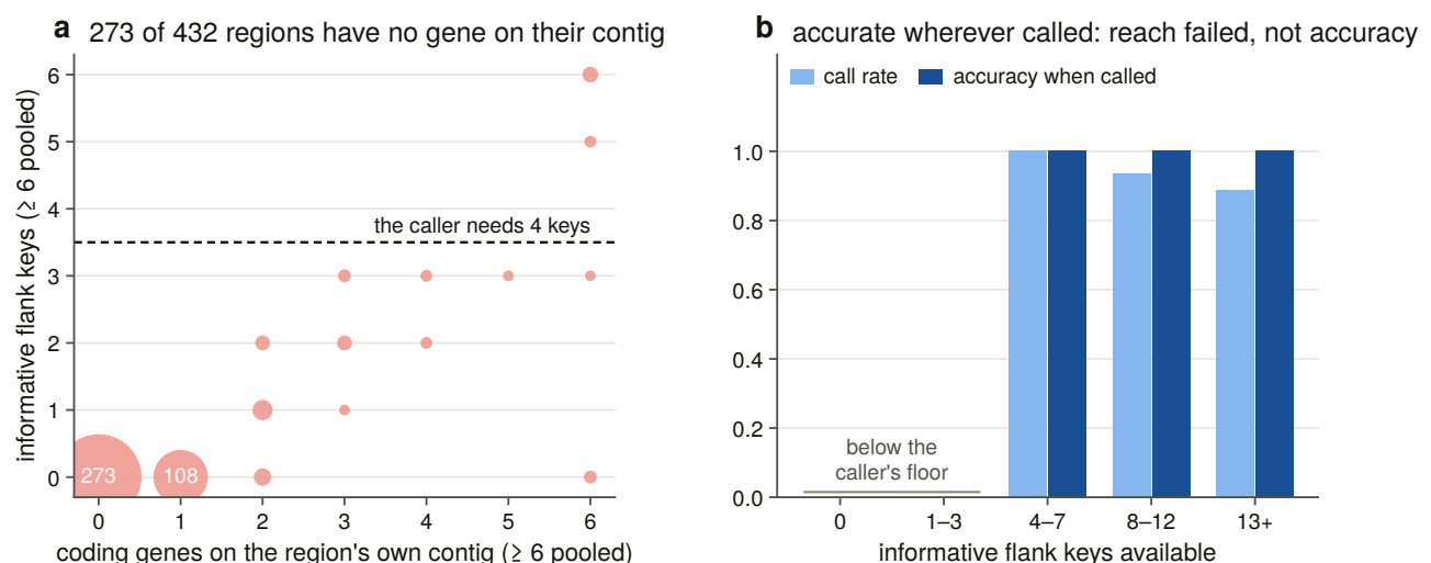
Figure 9.2. Synteny could not answer because a trace region has almost nothing to read. Panel a plots the joint distribution of coding genes and informative keys on each region's contig, with the caller's floor drawn, and panel b sets the caller's call rate and accuracy on the same key axis. The neighbourhood caller is right at every key count at which it acts, and it acts on 8 of 432 regions, because a fragment's contig carries no neighbours to read. Putting reach and accuracy on one axis is the only way to show that the method's failure here is a property of the data rather than of the method, which is what makes accurate and unavailable a readable verdict rather than an excuse.
