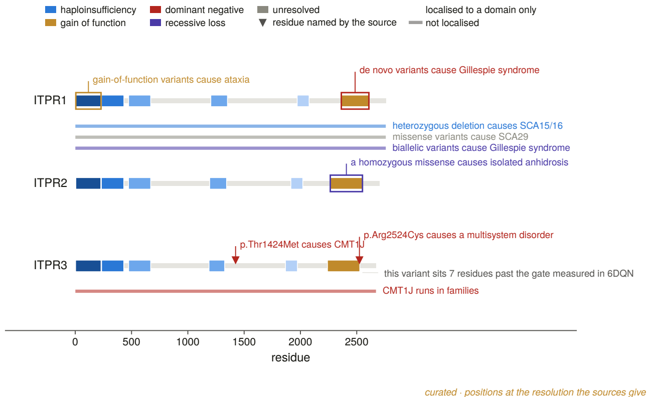
Figure 2.1. The curated disease-variant map records each variant as point, domain or gene according to how far its cited source actually localises it. That third column is the honesty of the figure: a source reporting a deletion of the whole gene cannot be drawn as a residue, and a map that drew it as one would assert a resolution the literature does not have. The distinction is what makes Chapter 11's variant analysis possible at all. A constraint map is scored against positions, and recording how far each source localises its variant is what showed that only two residue-level positions were available from the literature, which is why that chapter harvests a clinical database instead and uses those two as its positive control.
