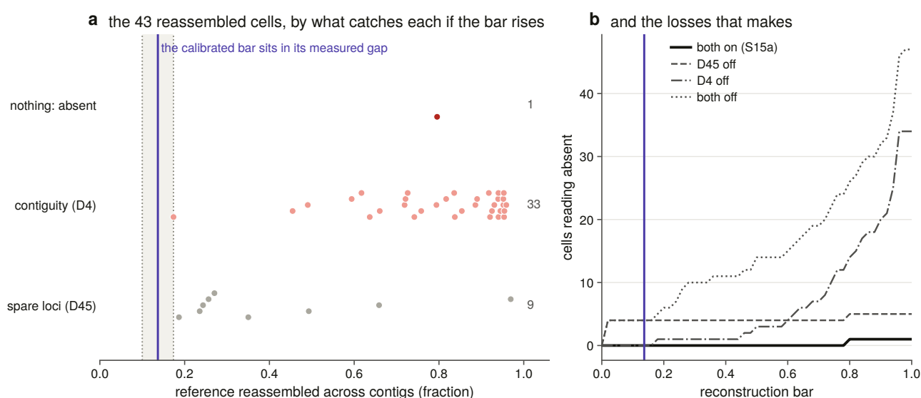
Figure 9.6. Each of the 43 reassembled cells is placed against the calibrated bar and its measured gap, on the row of the rule that would catch it if the bar rose, and panel b counts the cells that read absent as the bar is raised under each combination of the two protective rules. The within-row offset of each point is its rank in its own row, using no hash and no random number generator, so the figure is reproducible. Drawing both edges is what makes the threshold's own uncertainty visible, and the answer to the first sensitivity question is that moving the bar anywhere inside it changes no cell in 927.
