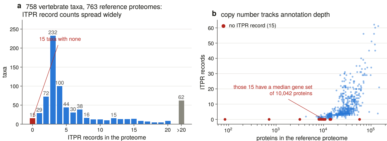
Figure 3.8. Copy number per proteome rises with annotation depth. (a) Calls per proteome are counted across the vertebrate taxa swept, with the fifteen that carry none marked. (b) Copy number is plotted against the size of each gene set. This relationship is the single strongest argument in the thesis for searching genomes rather than gene sets: a census built on reference proteomes measures how thoroughly each organism has been annotated at least as much as it measures how many receptors that organism has, and the correlation drawn here is that confound made visible. Every absence claim in this thesis is taken to an assembly for this reason, which is what Chapter 4 begins.
