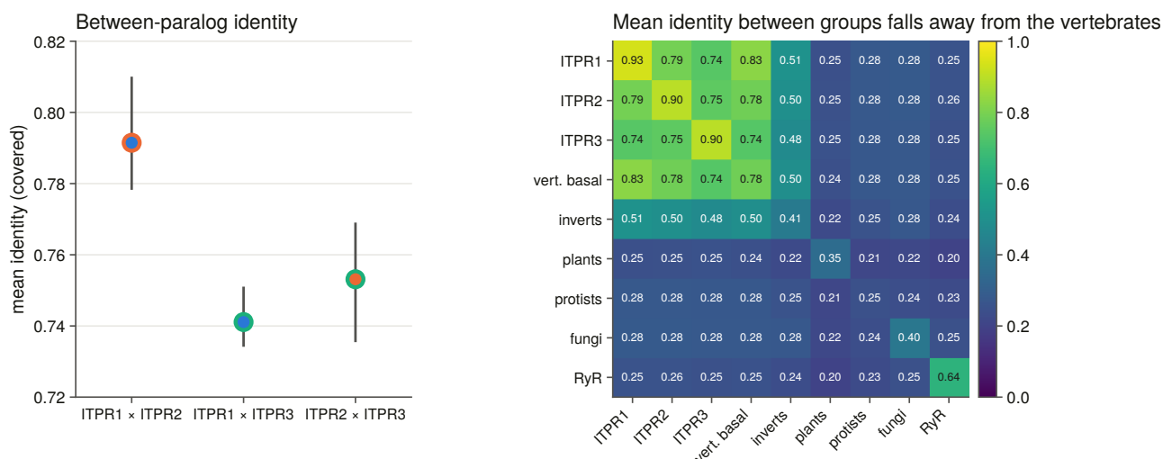
Figure 6.4. Identity within and between groups is summarised in two panels, the three paralogue pairs on the left and every group pair on the right. This figure fixes the scale every later comparison is read against: the three vertebrate paralogues sit at 0.74 to 0.79 to one another and at 0.91 within themselves, which is close enough that a bait from one aligns at all three genes. That single fact is why the duplication detector of Chapter 8 needed the family call before its geometry meant anything, and why the attribution margin inherited from a less similar family had to be overturned.
