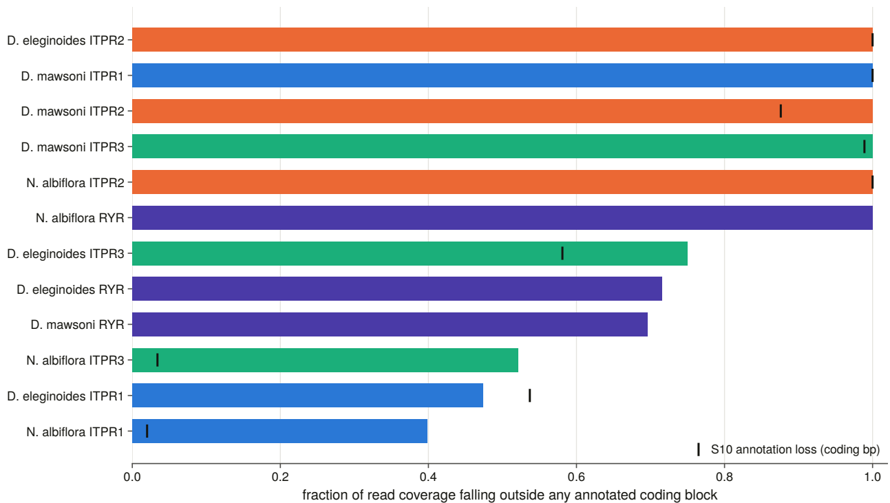
Figure 13.11. Read coverage over the sequence the annotation loses is the read-level form of the loss measurement. Each bar is the fraction of one locus's read coverage that falls outside any annotated coding block, for every locus in the panel including the ryanodine controls, and the tick on a bar is the coding footprint the exon-level measurement found no model delivering. Two independent instruments, one aligning a protein to a genome and one mapping reads to a spliced reference, are asked about the same missing sequence, and their agreement is what rules out the loss being an artefact of either.
