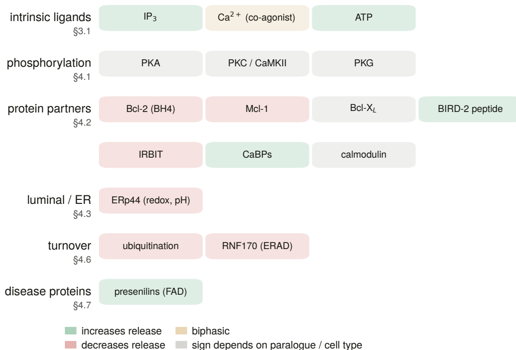
Figure 2.7. The curated regulator map shows what binds the receptor, where, and with what effect. It stands as a statement of scope rather than as a result, because it is the part of the biology this thesis does not measure. Nothing in a genome-scale census can say whether a protein interaction is conserved, so every measurement in this document passes this layer by, and the map is what a reader should weigh the census against.
