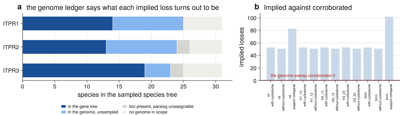
Figure 7.8. The genome ledger classifies each implied loss per paralogue, and the second panel sets the implied count in every cell of the matrix against the number the genomes corroborate. The figure is the reason a loss count is not read off a reconciliation: a reconciliation over a representative sample counts sampling, not biology. That is why Chapter 9 counts losses from 309 genomes instead, and why the two chapters' numbers are not alternative estimates of the same quantity.
