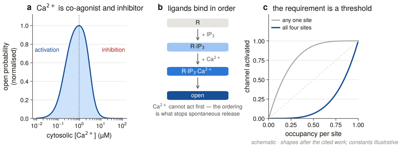
Figure 1.5. The figure draws what opens the channel and what closes it as logic rather than as mechanism. (a) Cytosolic calcium is both co-agonist and inhibitor, which is the bell-shaped dependence. (b) The two ligands bind in order, \text{IP}_3 first, so calcium cannot act on an unliganded receptor. (c) The requirement is a threshold rather than a single site. What matters for a census is what comes after this logic: the same channel produces puffs, waves and oscillations, and the properties that distinguish those outputs belong to the individual paralogue. If the three vertebrate paralogues were interchangeable, their copy number would be a matter of dosage and their individual retention would carry little information. Because they differ in affinity, in calcium sensitivity and in downstream output, the finding in Chapter 9 that all three are retained in every vertebrate genome is a statement about three distinct functions rather than about three copies of one.
