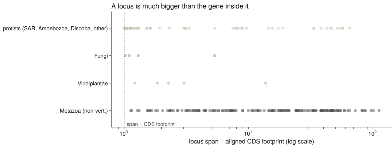
Figure 5.8. Locus span exceeds coding footprint by a factor that differs by group. The figure shows why a cluster of alignments is not a gene: a locus is much larger than the coding sequence inside it, and by a factor that varies roughly nine-fold between metazoan and protist genomes, so a single intron setting and a single contiguity bar would be far too lax for one group and far too strict for the other. This is the measurement behind the decision to set both per group, and behind the rule that a locus is not a copy.
