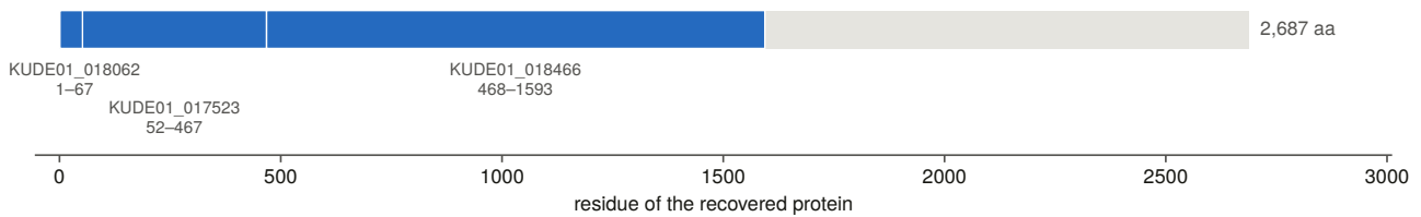
Figure 13.7. Tiling the annotated proteins back onto the genome's own recovered loci says whether the annotation missed a gene or broke it into pieces. Each panel is one case's recovered protein drawn as a bar, with the residues each annotated model delivers laid over it and the model named beneath. The proteins are translated from the assembly's own annotation and genome rather than downloaded, because a locus filed as a pseudogene emits no protein record and those loci are exactly the ones under dispute. The guard that matters is that the subject set is the genome's own loci: a query whose own locus is missing from that set lands on its nearest paralogue instead, and the row then reads as a confident naming disagreement, which is exactly what happened before the check existed.
