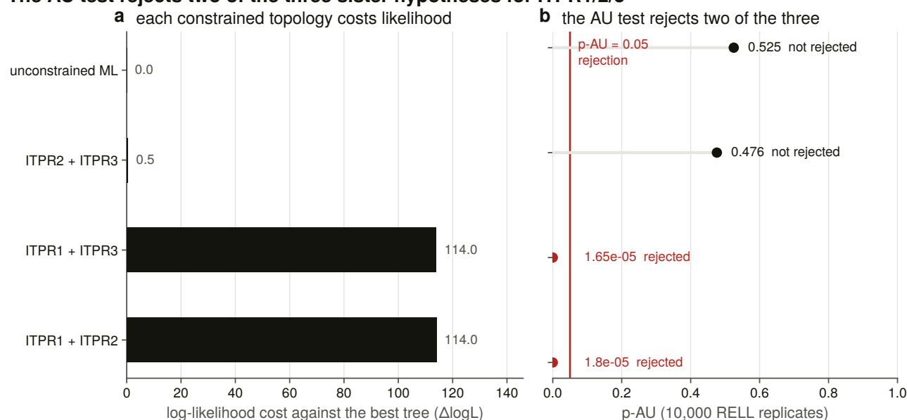
Figure 6.8. The three sister hypotheses are compared under the approximately unbiased test [55], with the log-likelihood difference and the p-value on two panels sharing one row of categories rather than on two y-axes. They are different measures on different scales, and a twin axis invites a comparison that has no meaning. This figure is the answer to Chapter 6's central question, and its importance is that it excludes rather than merely prefers. Two of the three possible sister arrangements fall outside the 95 % confidence set of topologies for this alignment, at p below 2 \times 10^{-5} , so the result is not a ranking that a slightly different alignment could reverse. Chapter 7 then shows the genomic neighbourhood pointing the other way, and the two are reported as a disagreement rather than reconciled.
