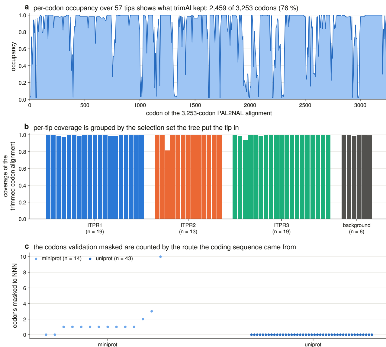
Figure 10.1. The trimmed codon alignment carries every estimate in this chapter, and the figure is plotted in codons because an axis in nucleotides would make a three-fold difference look like a property of the data. The three panels show per-codon occupancy across the 57 tips (a), the coverage of each tip by the selection set the tree placed it in (b), and what validation masked, by the route each coding sequence came from (c). A reader can therefore see the size of what every rate in Chapter 10 was estimated on, which is 2,459 codons of 3,253 after trimming, across 57 tips whose coding sequences were each proved to encode the aligned protein.
