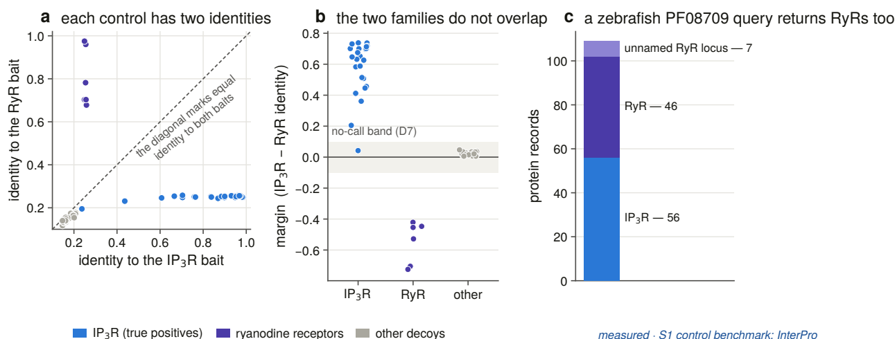
Figure 2.4. The families are separated by evidence rather than by name, using the control panel Chapter 3 builds. Panel a shows every control scored against a labelled IP 3 receptor bait and a labelled ryanodine receptor bait, and the two families fall on opposite sides of the diagonal with nothing between them. Panel b shows the same data as a margin, with the band inside which this project declines to call either way drawn rather than described. The one positive inside that band is Dictyostelium iplA, a characterised receptor that the family's own defining signature does not find. Panel c shows the zebrafish query and the 53 records in it that are the sister family. The importance of the gap in panel b is that it is what every later instrument had to reproduce. A margin with no gap would mean the two families cannot be separated by sequence, and every downstream count would then be a mixture of both. The one positive inside the no-call band is equally important in the other direction, because it shows that this instrument cannot reach the deepest branches, which is why the profile models of Chapter 3 exist.
