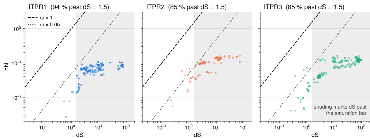
Figure 10.3. Pairwise rates within each paralogue reach synonymous saturation, and the three panels draw them log-log with the neutral diagonal and the saturation bar. On a logarithmic-x, linear-y plot the neutral diagonal is not a line at all: the first draft's neutrality ran off the panel within the first pixel and left the saturation bar as the only line on the figure, which reads as neutrality. What the panel shows is that saturation is reached inside a single paralogue and not only between the three, which is the reason no rate in this chapter is taken from a pairwise matrix.
