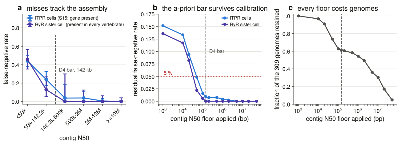
Figure 4.5. The false-negative rate falls with assembly contiguity in both control series, and the bar is drawn where the a-priori floor sits. This is the figure that licenses the retention result, because a survey reporting zero losses is worth nothing unless somebody has measured how often the same search fails to find a gene that is demonstrably present. The two series are independent, since the ryanodine sister series uses none of the state rules the family series depends on, and they agree, which is what stops the number being read as the search agreeing with itself.
