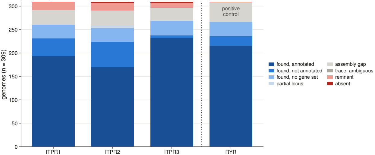
What the genomic sweep found, per paralog
