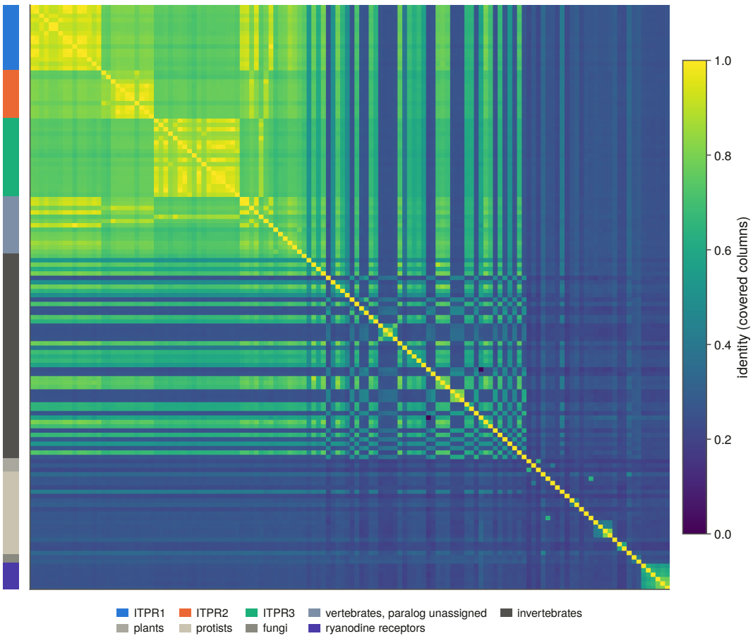
Pairwise identity over mutually covered columns, 134 representatives
