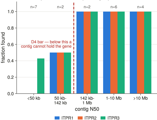
a Recovery tracks assembly contiguity
