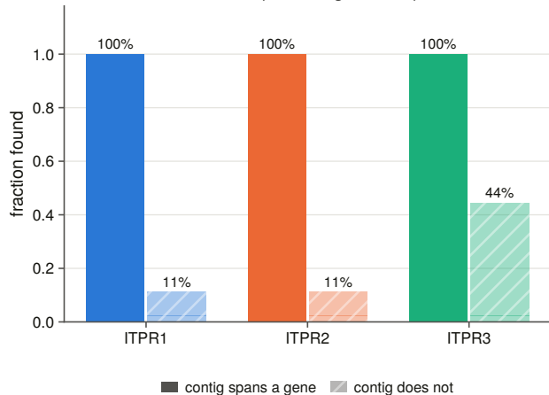
b Either side of the bar (12 vs 9 genomes)
