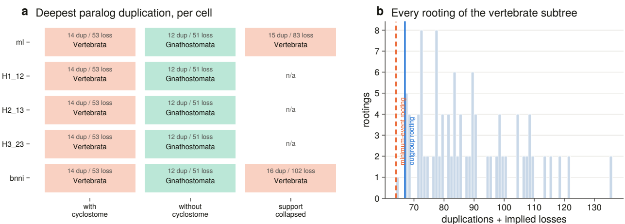
Figure 7.10. The topology \times variant matrix, with the deepest paralogue duplication in every cell, and beside
