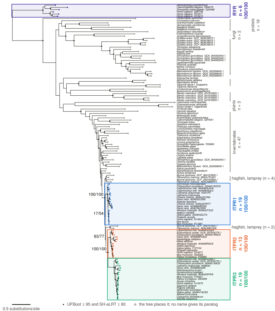
The maximum-likelihood tree of 134 family proteins recovers ITPR1, ITPR2 and ITPR3 as clades, rooted on the ryanodine receptors
