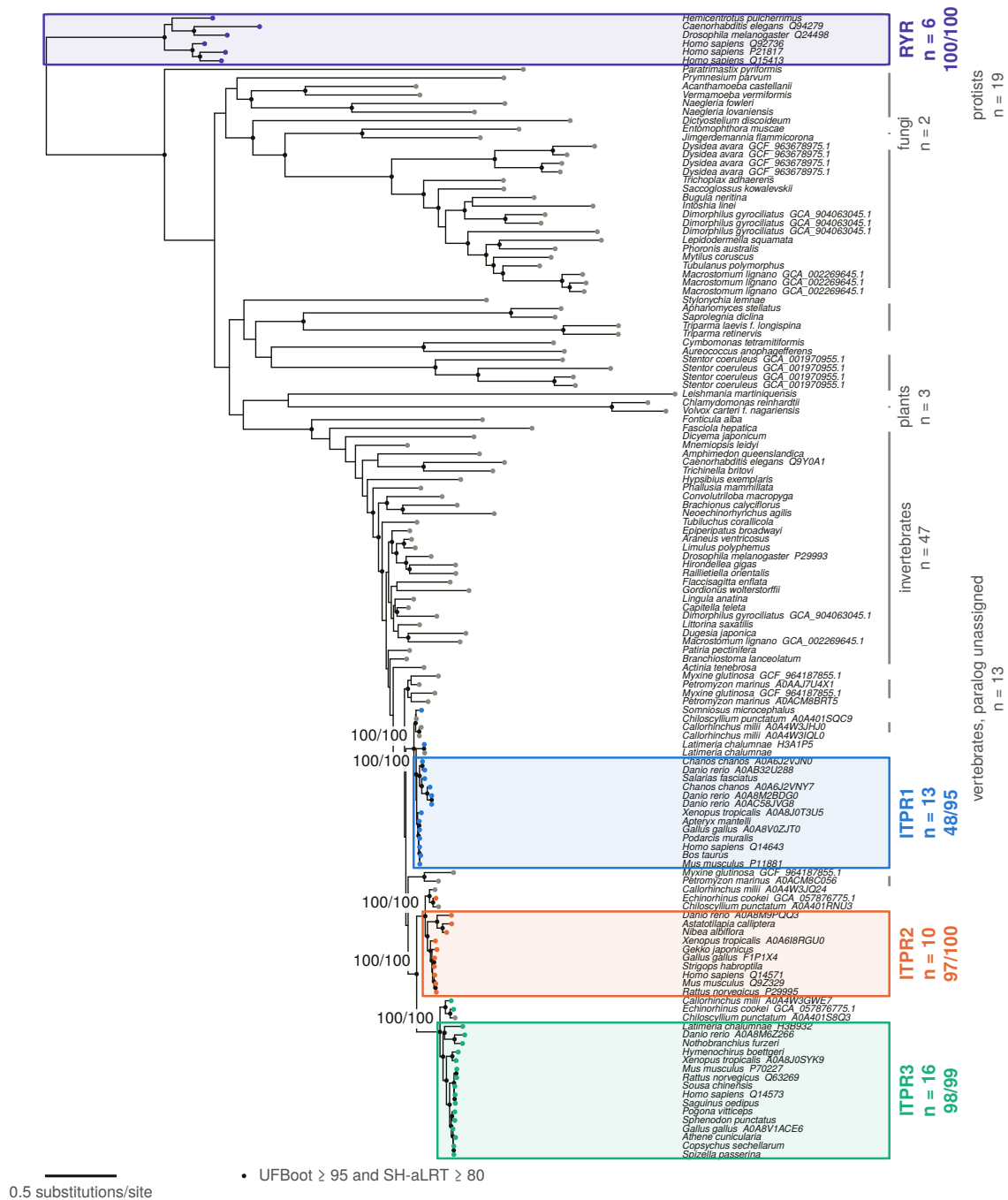
Fig. 3 | One family, three vertebrate paralogues, rooted on the ryanodine receptors. Maximum-likelihood phylogram of 134 representative proteins over 1,797 trimmed alignment columns under Q.insect+R7, rooted on the six ryanodine receptor sequences. Coloured boxes mark the three vertebrate paralogue clades and the outgroup, each labelled with its tip count and its SH-aLRT/UFBoot support; the vertical bars on the right name the taxonomic grades of the tips outside them. Filled circles mark nodes clearing SH-aLRT \geq 80 and UFBoot \geq 95 . The five 100/100 labels on the backbone are the two ancestors of each boxed clade: the three extended paralogue clades — each core clade plus the basal vertebrate tips the tree nests with it — an inner ITPR1 node of 15 tips, and, deepest, the 32-tip node uniting ITPR2 and ITPR3 . Scale bar 0.5 substitutions per site.
