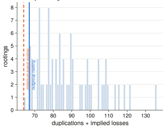
b Every rooting of the vertebrate subtree
