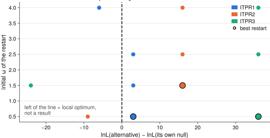
Branch-site model A: every restart against its null
