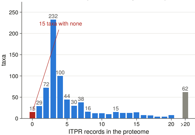
a 758 vertebrate taxa (763 reference proteomes)
