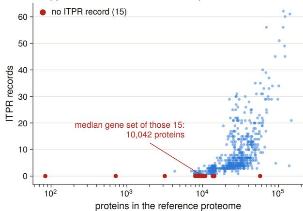
b copy number tracks annotation depth
