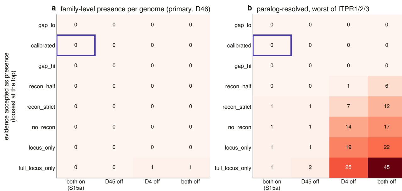
Dollo losses manufactured by each setting of the rule chain (309 vertebrate genomes); the violet ring is S15a's own operating point
