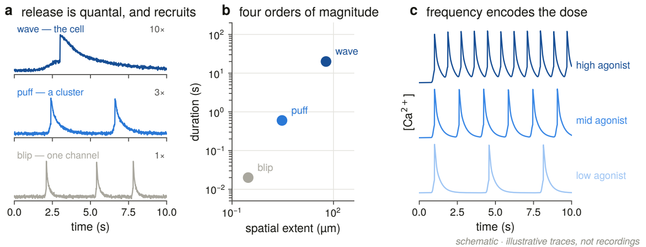
Figure 1.4. How the calcium signal is built, and what carries the dose. (a) The three event classes, drawn as illustrative traces rather than recordings: a blip is one channel opening, a puff is a cluster of them, and a wave is the cell. Each has its own amplitude band, because the blip is roughly ten times smaller than the wave and one shared axis would draw it as a flat line. (b) The same three events placed by how far they spread and how long they last, which is four orders of magnitude on each axis. (c) Raising the agonist raises the frequency of the events rather than their size, so the dose is carried in the timing. The figure is here to mark the boundary of what follows: everything in this thesis is a statement about the gene and the protein, and nothing in it reaches panel c.
