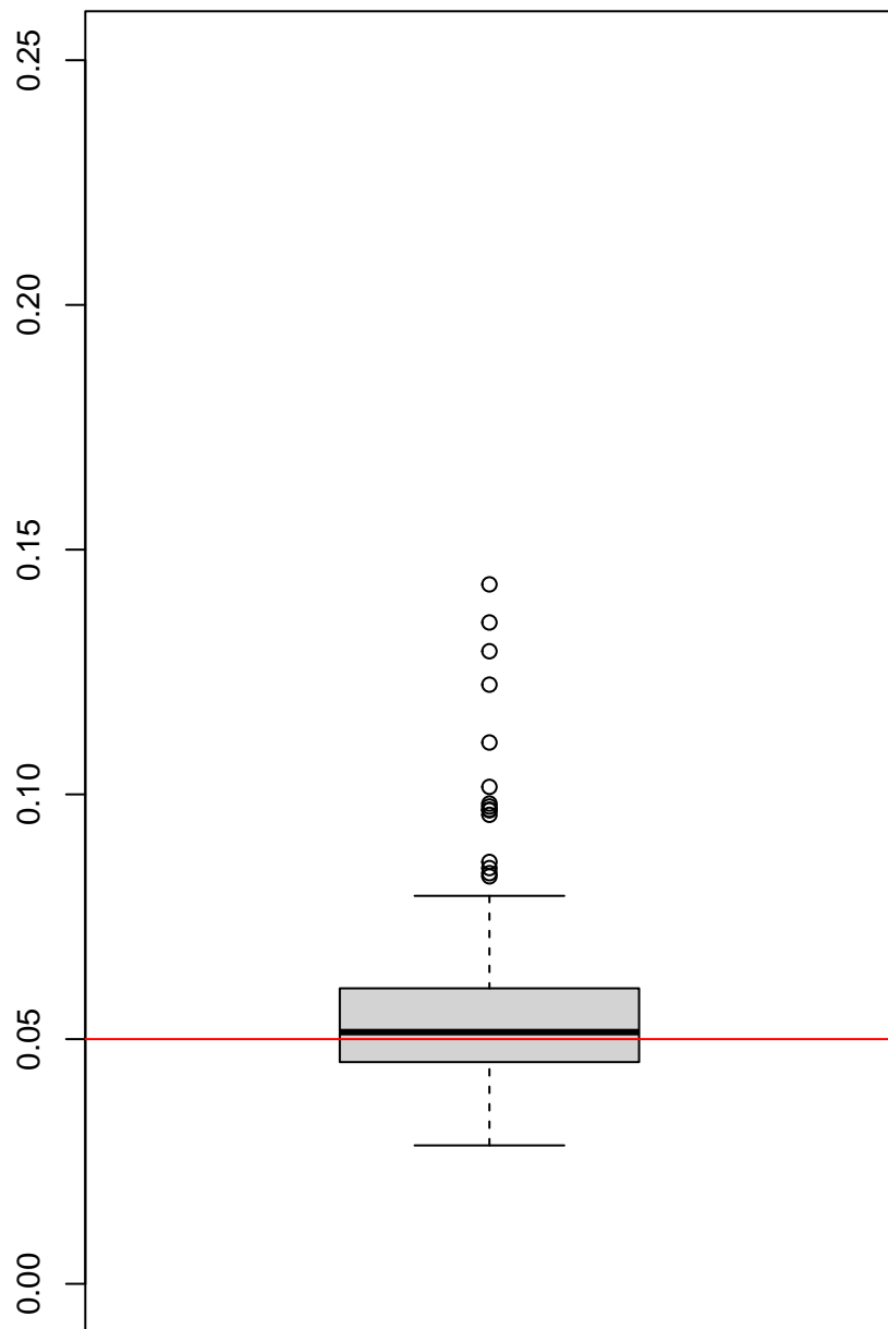
Strata 1 Density estimates
