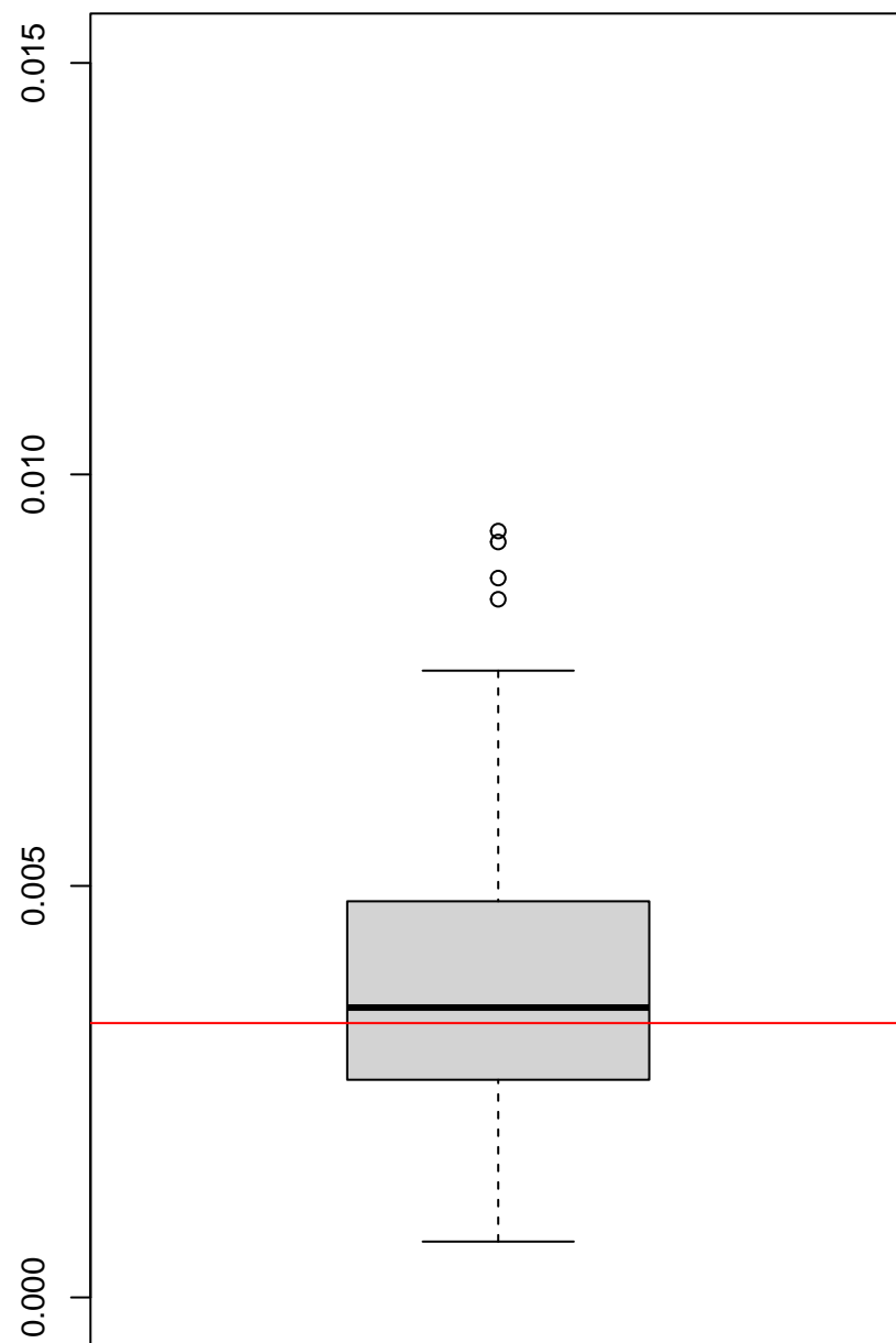
Strata 2 Density estimates
