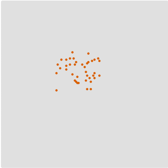
\min(n,r) G_2
