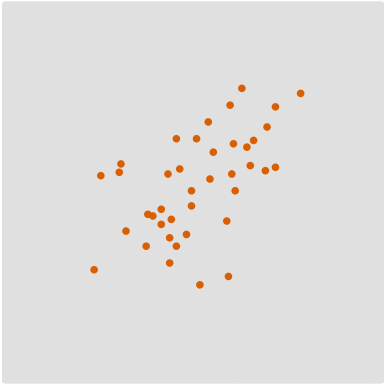
\min(n,r) \text{ Avg}
