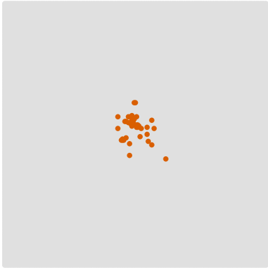
\min(n,r) \text{ Both}
