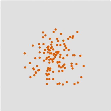
\min(n,r) \ G_2
