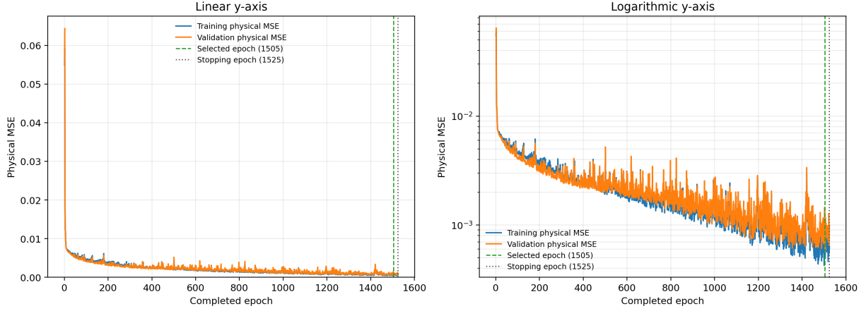
Figure 32: Physical training and validation MSE for the final production run. The left panel uses a linear y-axis and the right panel uses a logarithmic y-axis; both contain all 1525 completed epochs. The dashed line marks the selected epoch 1505 and the dotted line marks the stopping epoch 1525. Both panels use physical-unit MSE, while the standardized SIMM objective is not shown.
