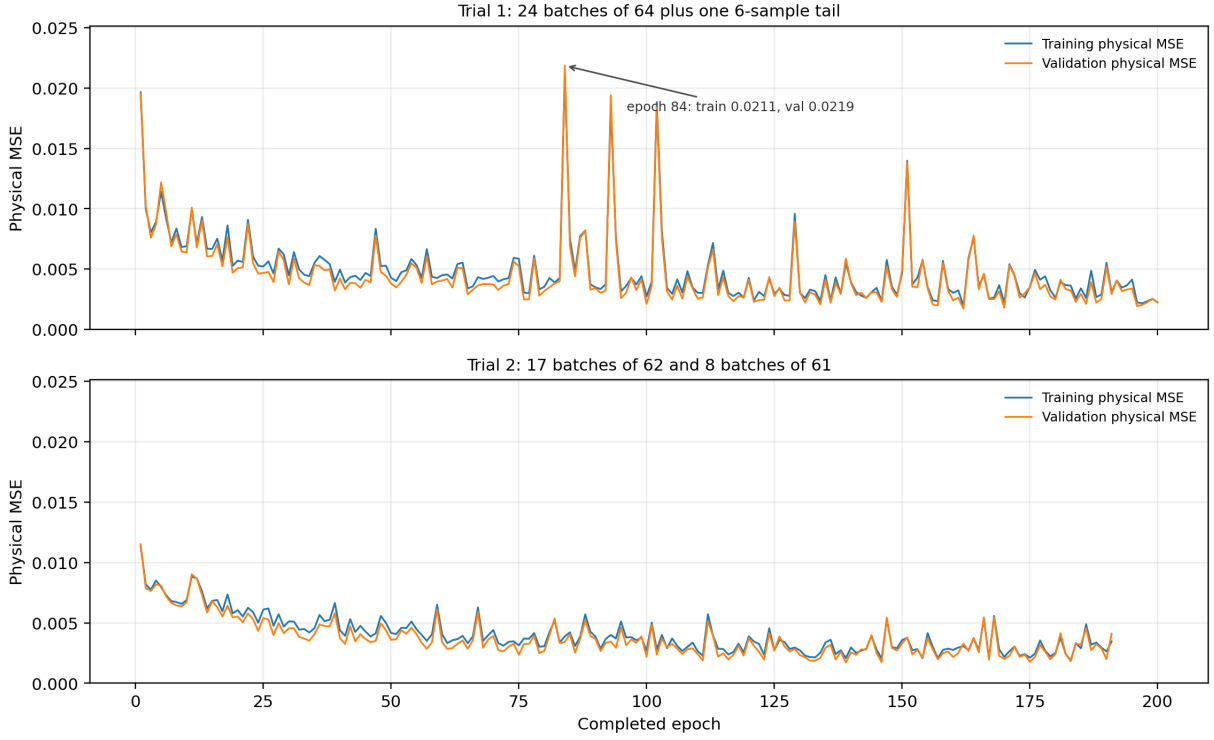
Figure 32: Physical training and validation MSE for the two seed-42 runs at global batch size 64. The upper panel is trial 1 with 24 batches of 64 plus a 6-sample tail; the lower panel is trial 2 with 17 batches of 62 and 8 batches of 61. The common linear scale includes the full histories of 200 and 191 completed epochs. The annotation marks the epoch-84 excursion in trial 1. These are single-run histories, not fold averages; the standardized SIMM objective is not shown.
