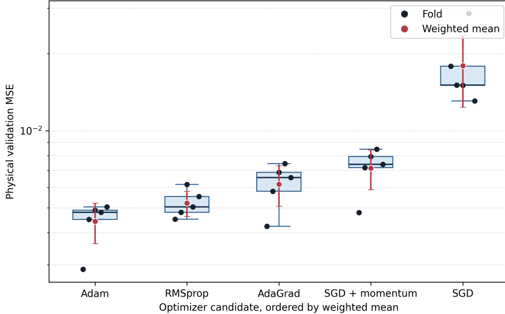
Figure 19: Optimizer ranking from the five-fold comparison at learning rate 10^{-5} . Dark points are individual physical validation MSE values, boxes summarize the five folds, and red points with bars show the sample-weighted mean and weighted population standard deviation. The vertical axis is logarithmic.
