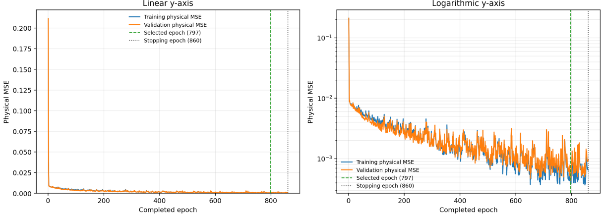
Figure 34: Physical training and validation MSE for production_slurm-56688223 . The left panel uses a linear y-axis and the right panel a logarithmic y-axis; both contain all 860 completed epochs. The dashed line marks selected epoch 797 and the dotted line stopping epoch 860. The standardized SIMM objective is not shown.
