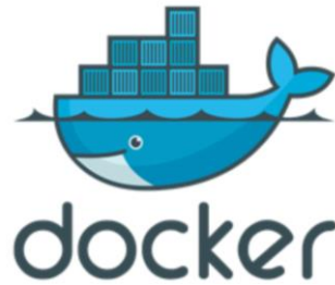
docker
