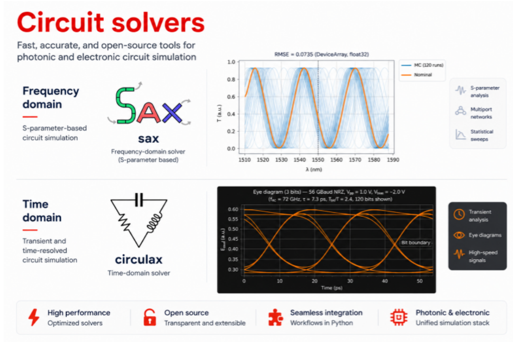
Figure 4. Circuit solvers for photonic and electronic circuit simulation: SAX for frequency-domain, S-parameter-based analysis, and Circulax for time-domain, transient simulation.
