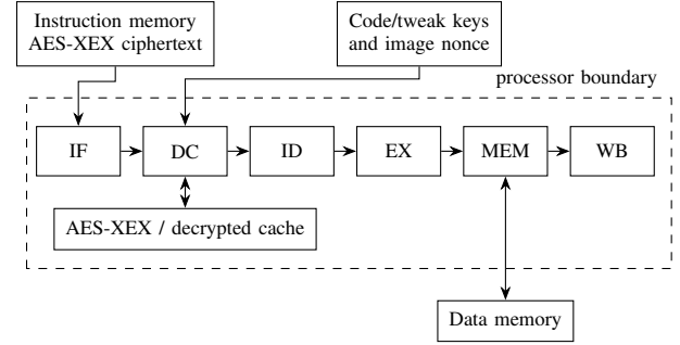
Fig. 1. Logical instruction path. Plaintext instruction blocks remain inside the core. AES data instructions operate through MEM using a separate data key.
