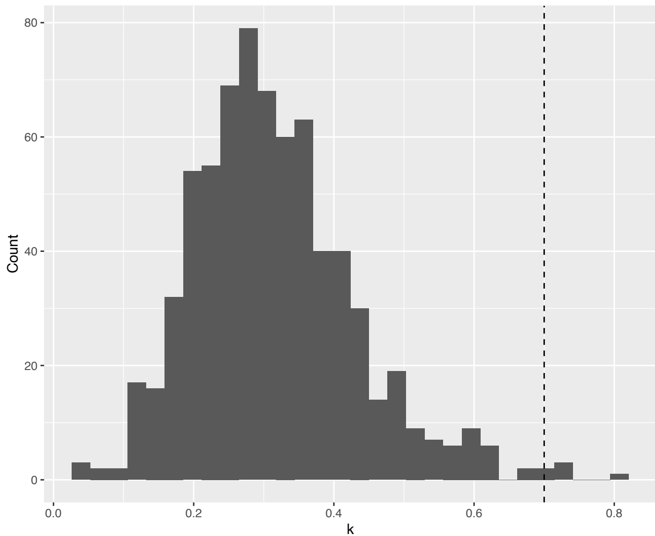
Pareto-k histogram
