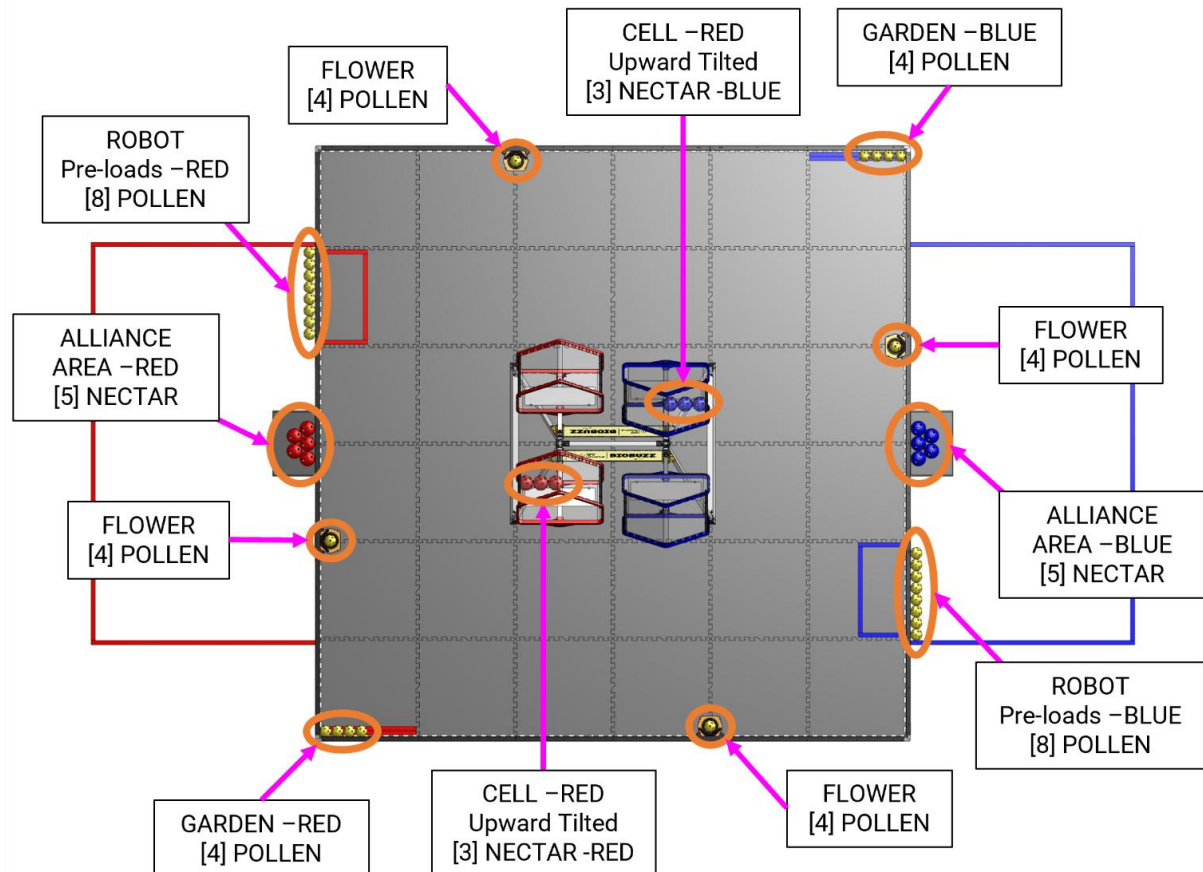
Figure 10-2: SCORING ELEMENT staging positions
