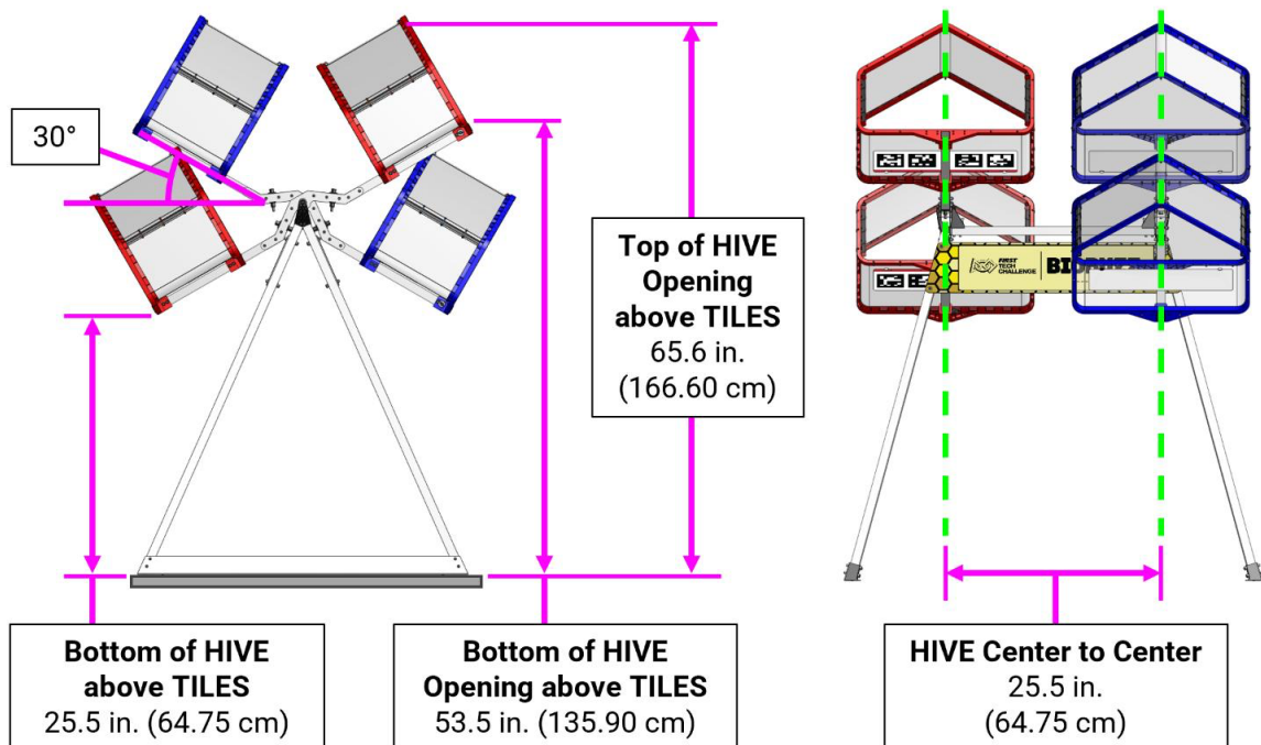
Figure 9-10: HIVE and CELL Key Details
