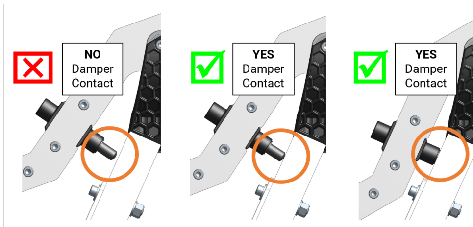
Figure 10-3: HIVE damper and frame
