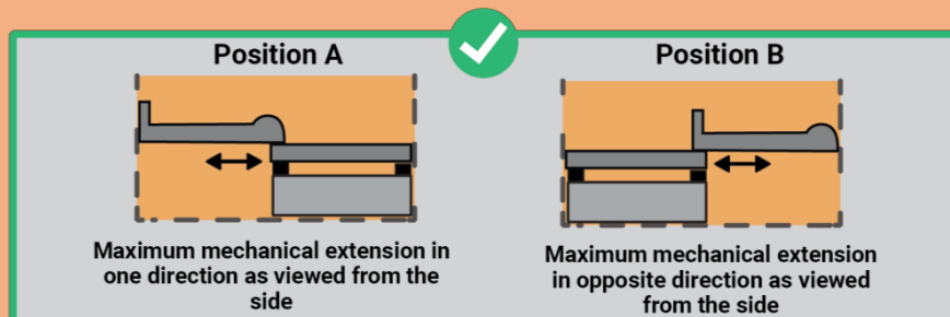
Figure 12-4: Expansion Limit – Allowable Extension
