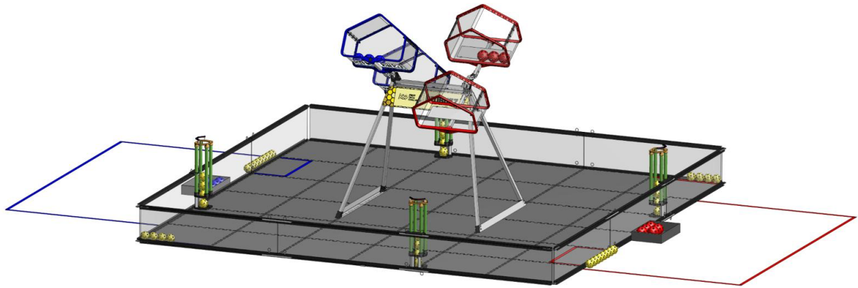
Figure 10-1: FIELD for BIOBUZZ
