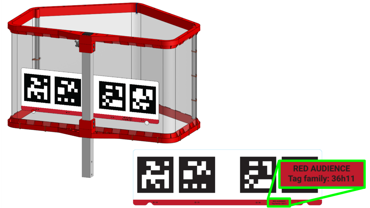
Figure 9-16: AprilTag Cluster on CELL
