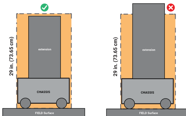
Figure 12-2: Expansion Limit – Side View
