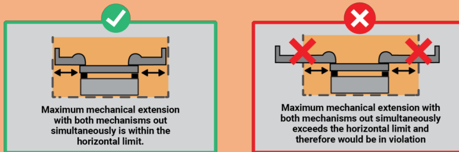
Figure 12-5: Expansion Limit – Simultaneous Extension
