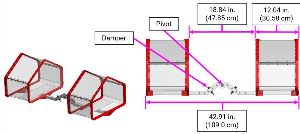
Figure 9-10: HIVE and CELL Key Details
