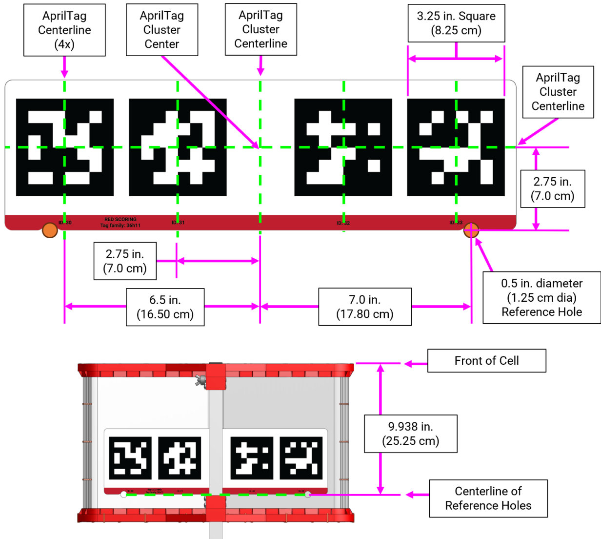
Figure 9-15: AprilTag Cluster and Reference Hole layout
