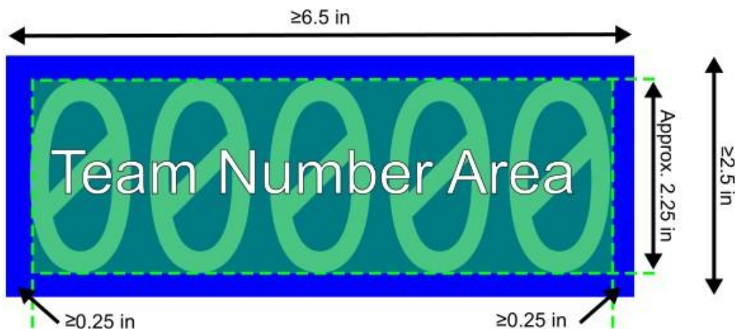
Figure 12-7: Team Number ROBOT SIGN Sizing
