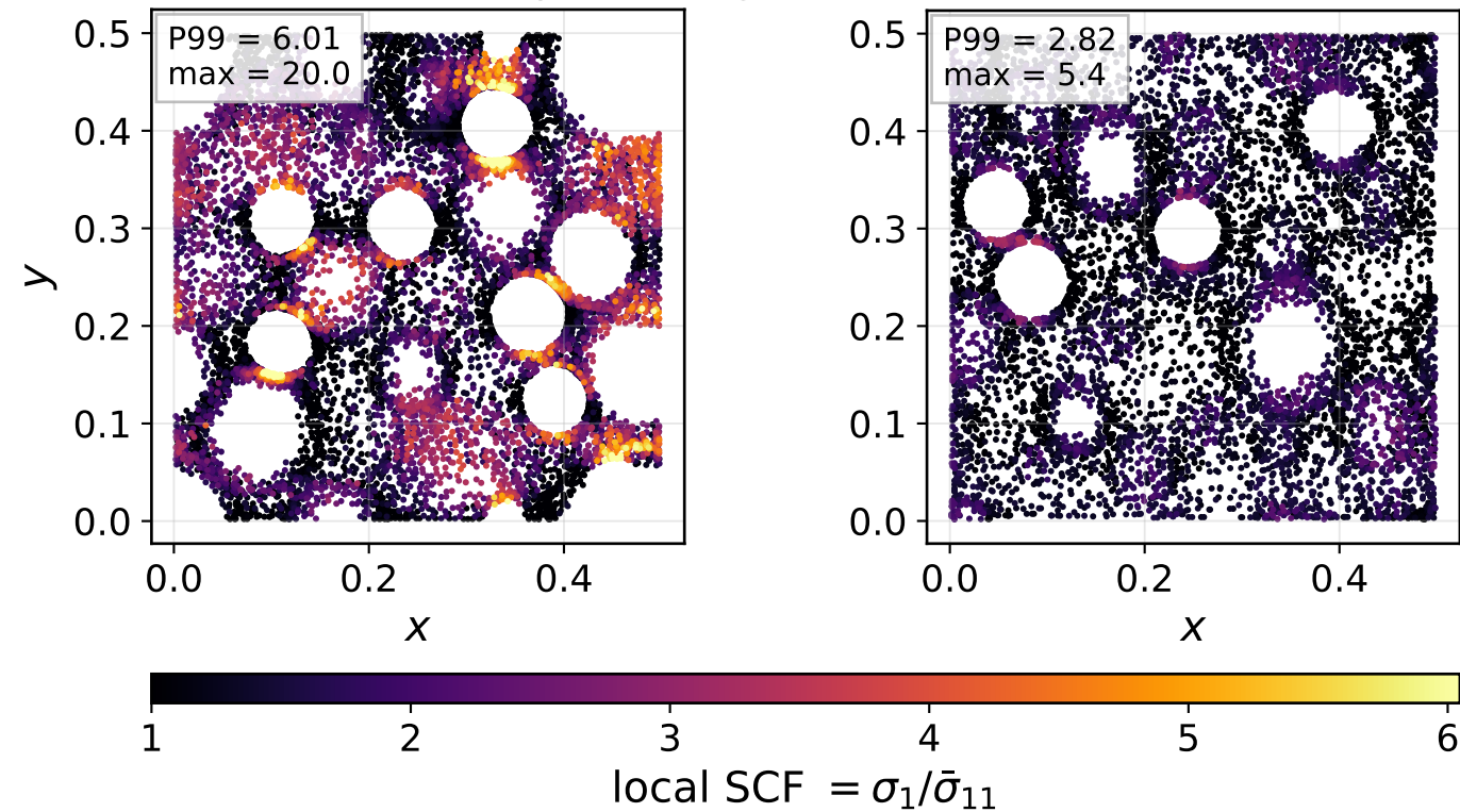
(a) warm base (channels + pockets + gas)
