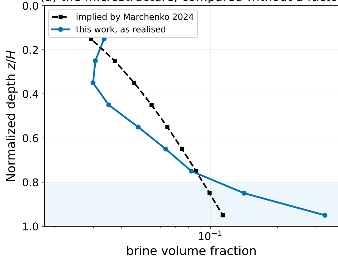
(a) the microstructure, compared without a factor
