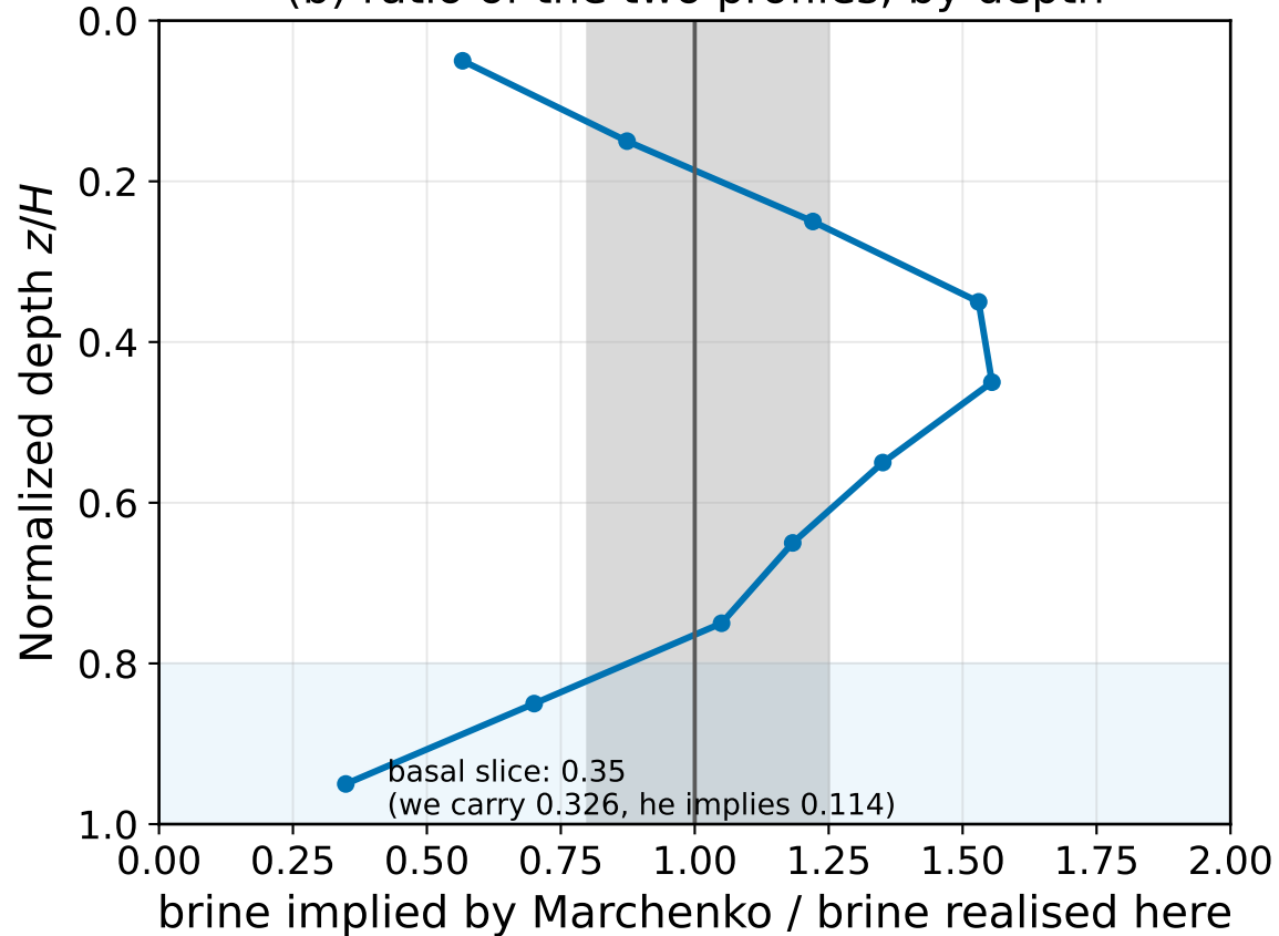
(b) ratio of the two profiles, by depth
