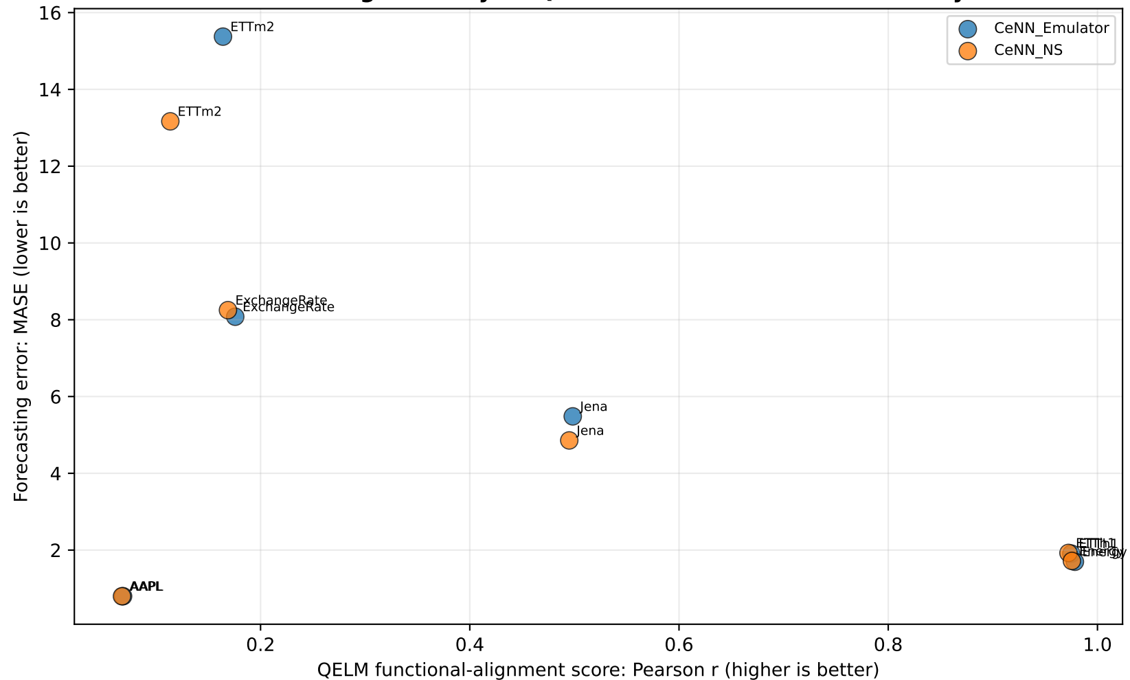
Forecasting accuracy vs QELM functional-emulation fidelity
