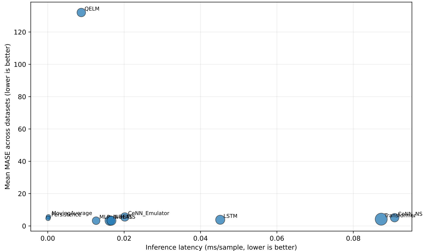
Accuracy-efficiency trade-off
