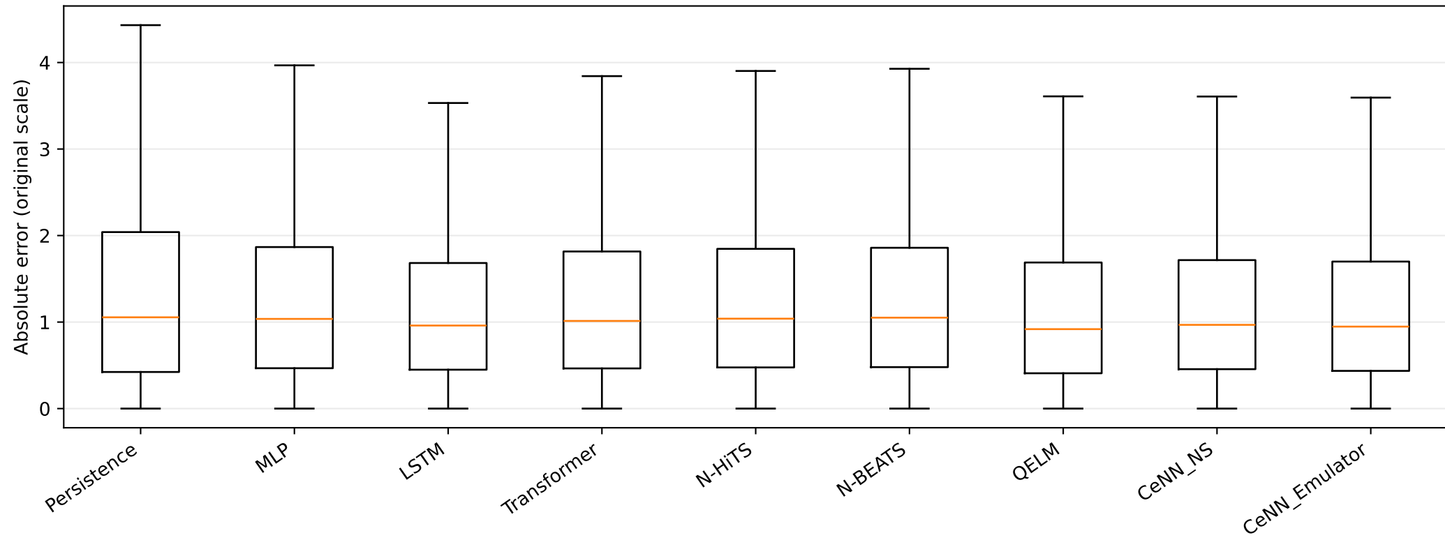
Supplementary diagnostic — ETTh1 absolute-error distribution
