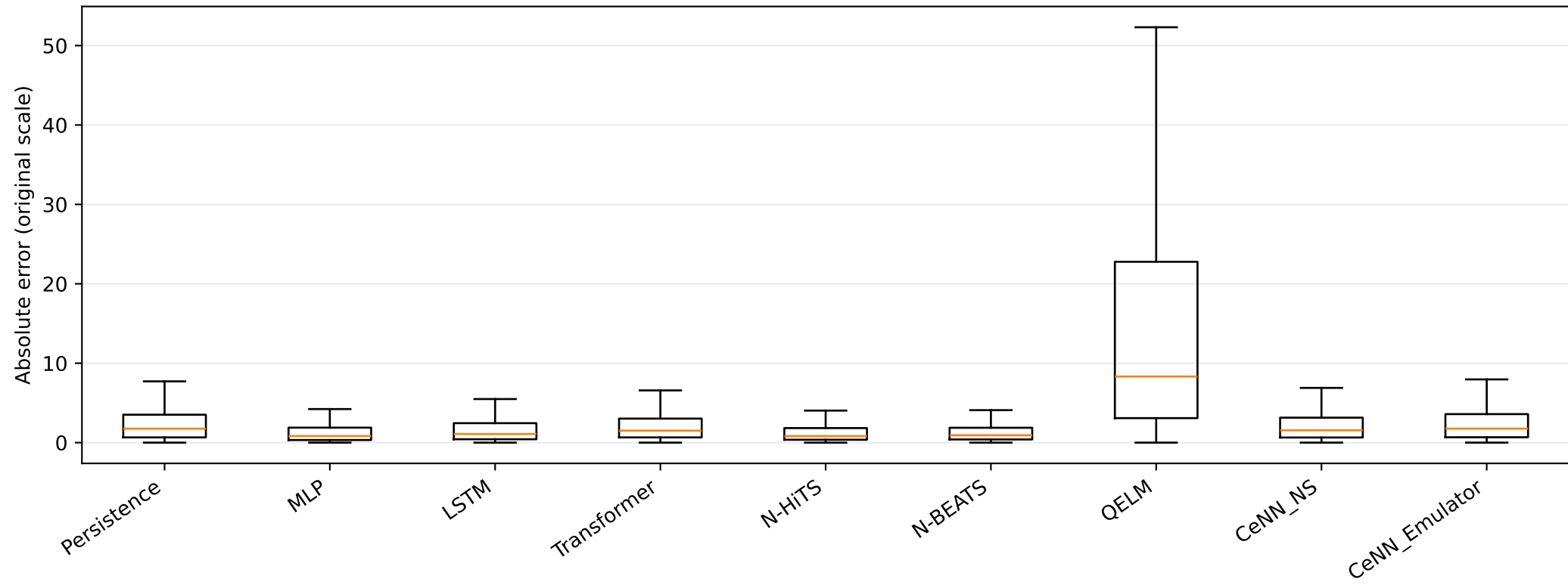
Supplementary diagnostic — ETTm2 absolute-error distribution
