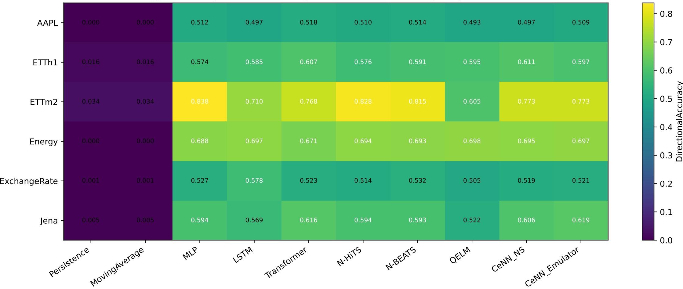
Supplementary metric heatmap — DirectionalAccuracy (higher is better)
