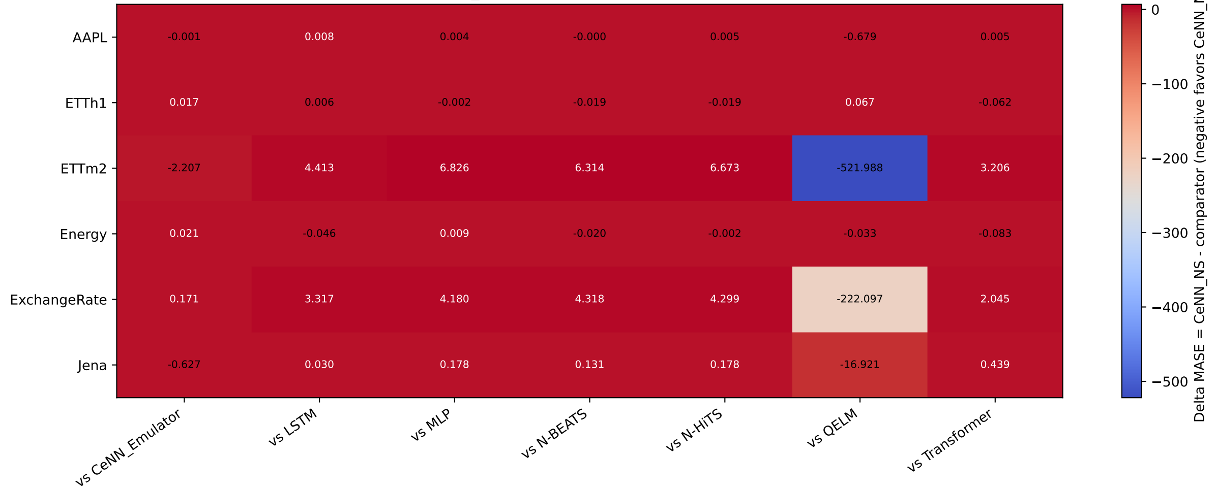
Paired comparison summary — CeNN_NS vs selected baselines (Wilcoxon p-values available in CSV)
