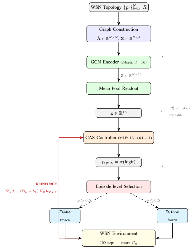
Fig. 1: GAPF architecture (CAS mode). Sensor positions and communication radius define a graph encoded by a two-layer GCN with mean-pool readout ( \mathbf{z} \in \mathbb{R}^{16} ). The CAS controller maps \mathbf{z} to a selection probability p_{\text{QMIX}} . The chosen frozen expert executes the full episode. The return G_k feeds back (red arrow) as a REINFORCE signal to update only the 1,473 meta-controller parameters.
