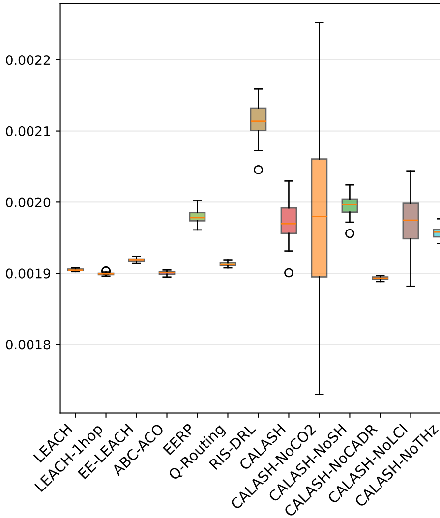
Total Carbon gCO 2 (↓)
