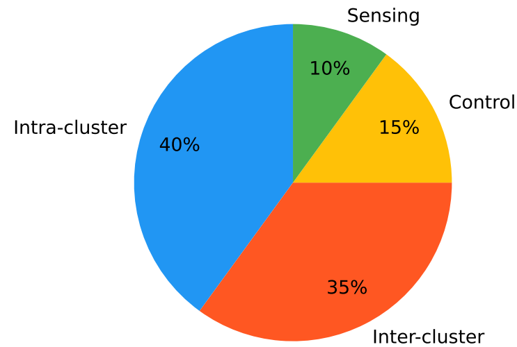
LEACH
