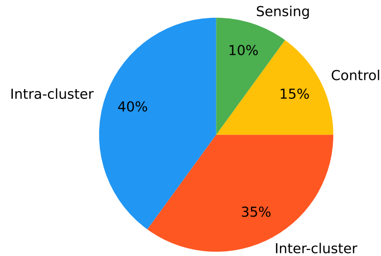
CALASH
