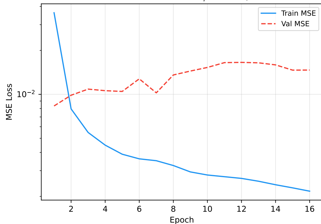
(c) Contrastive Safety Encoder ( q_\phi , \sim 8K params)
