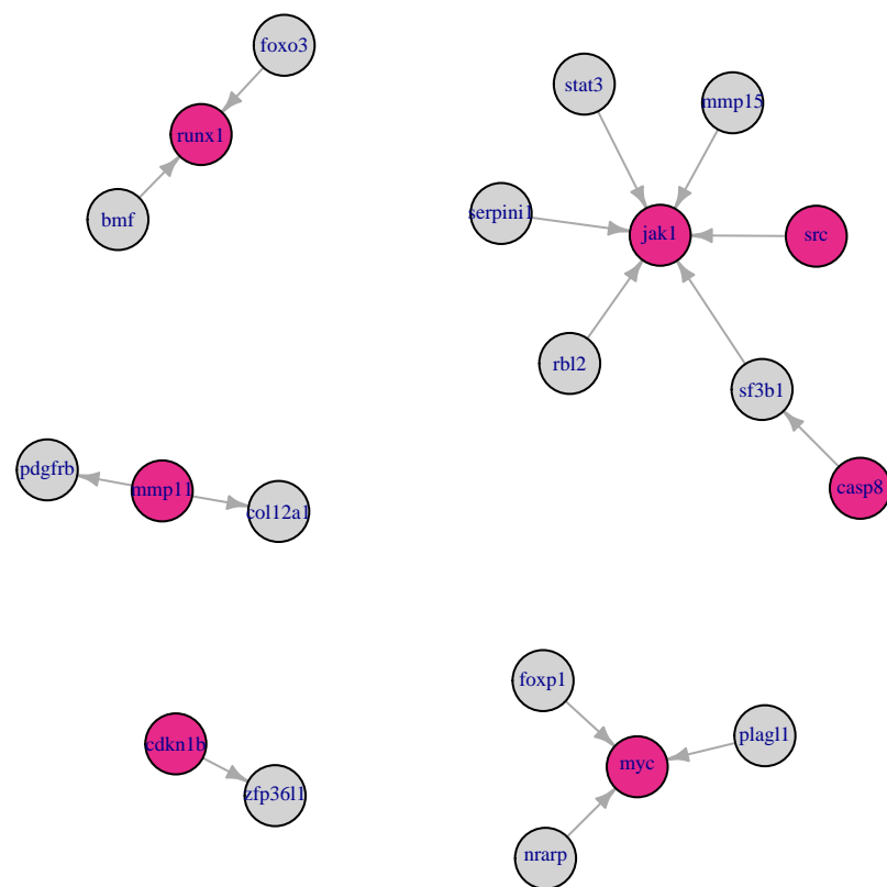
BASAL – Driver Gene Causal Network
