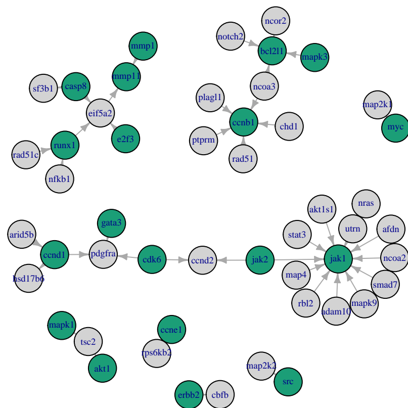
LUMA – Driver Gene Causal Network
