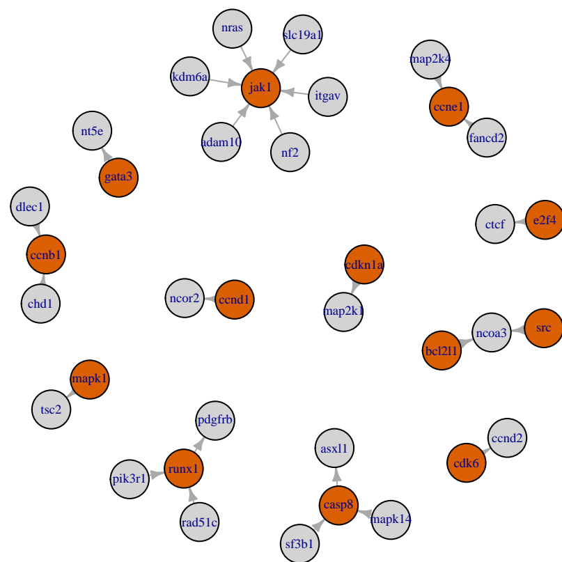
LUMB – Driver Gene Causal Network
