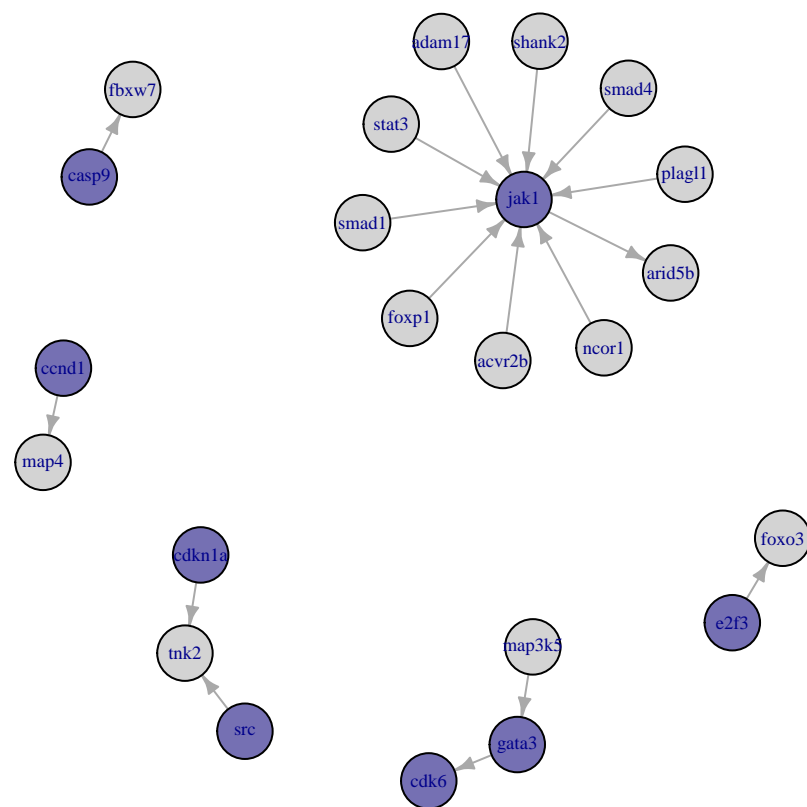
HER2 – Driver Gene Causal Network
