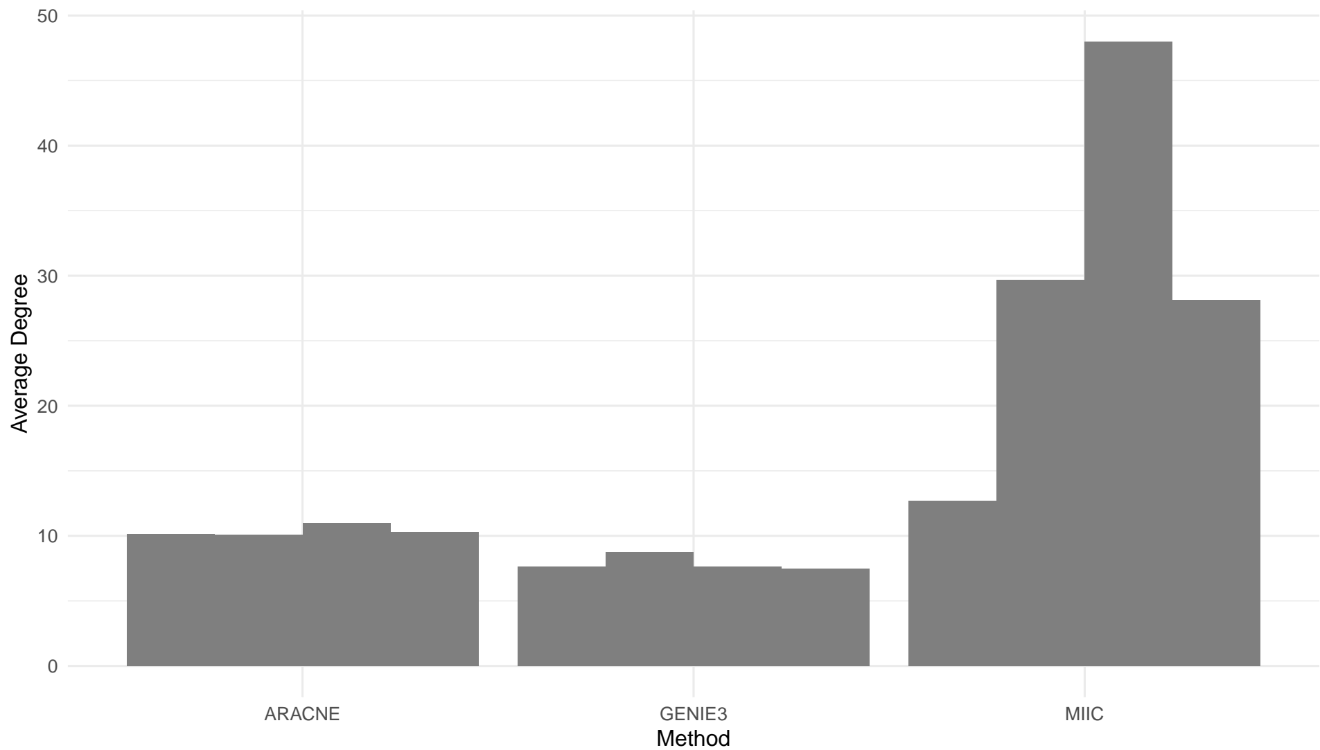
Average Node Degree by Method and Subtype
