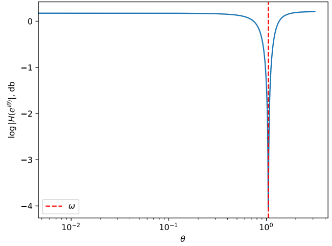
Figure 5: Notch filter frequency response
