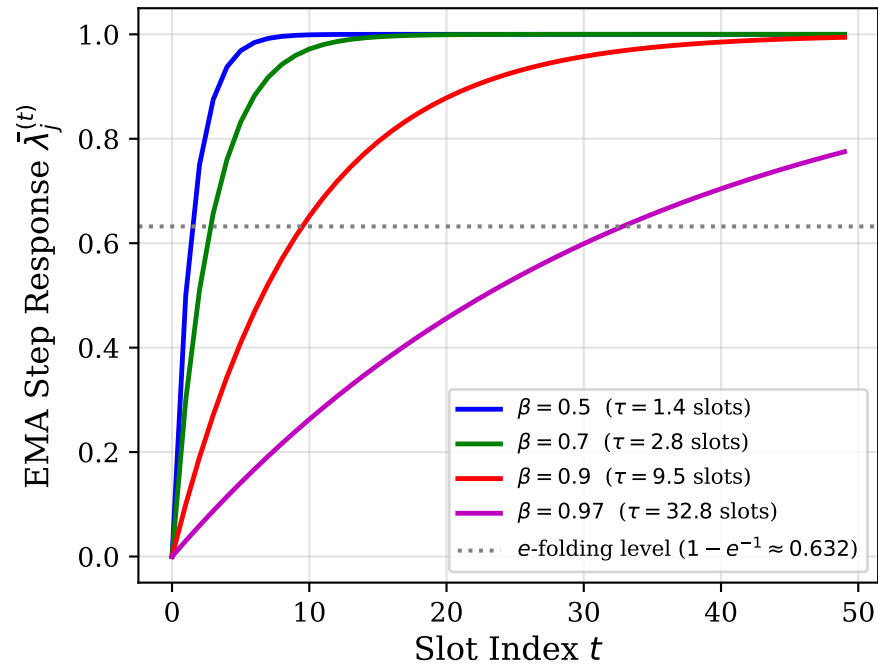
(b) EMA Step Response (Proof of Proposition~\ref{prop:beta})
