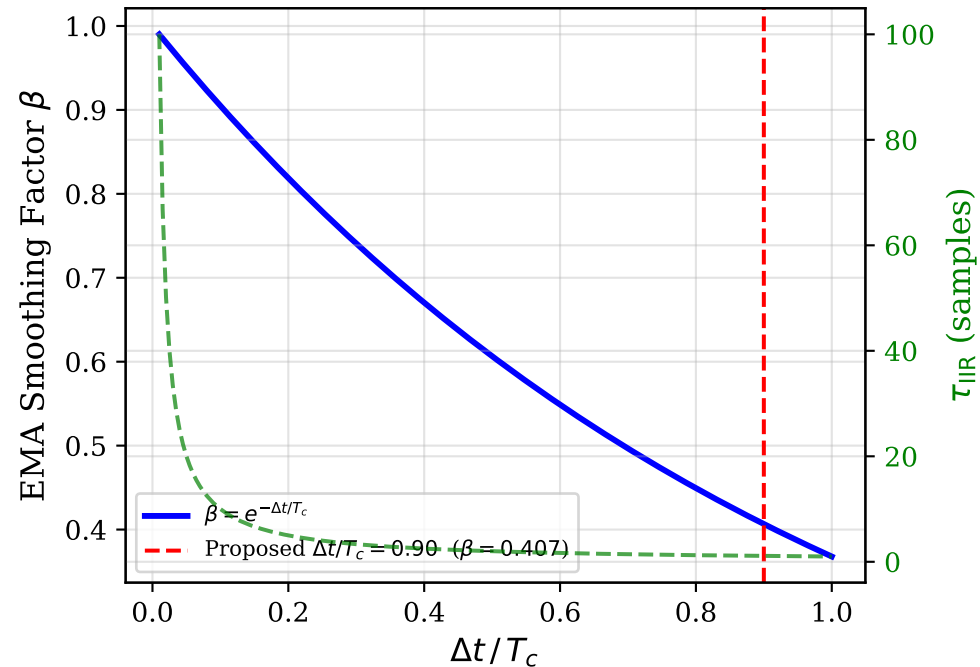
(a) \beta Derivation (Proposition~\ref{prop:beta})
