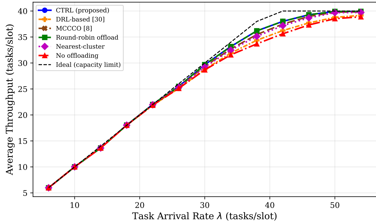
System Throughput vs Offered Load
