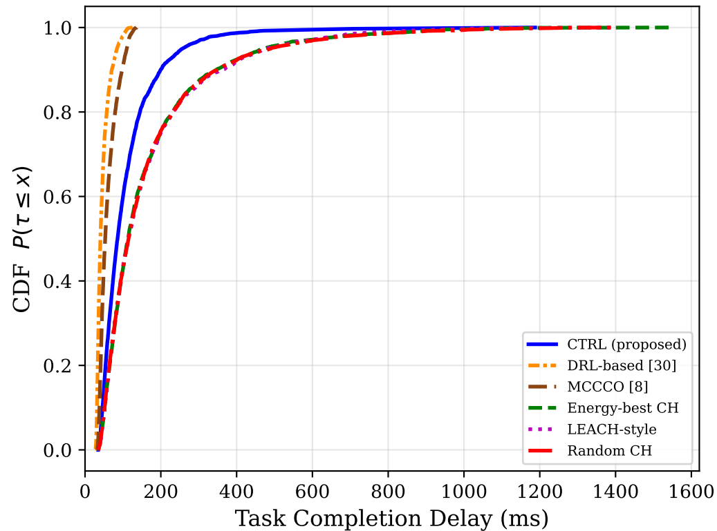
(a) Delay CDF ( N = 20 UAVs)
