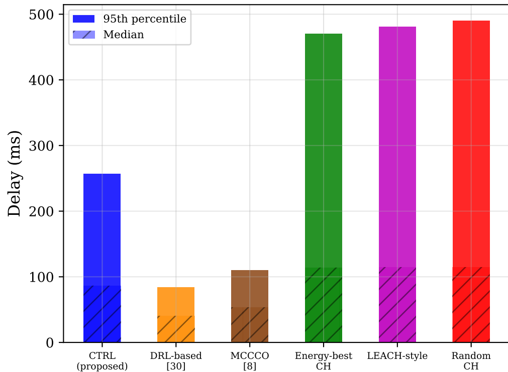
(b) Median and 95th-Percentile Delay
