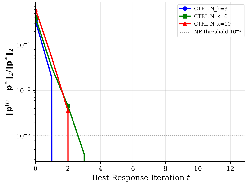
(a) CTRL: BR Game Convergence to NE
